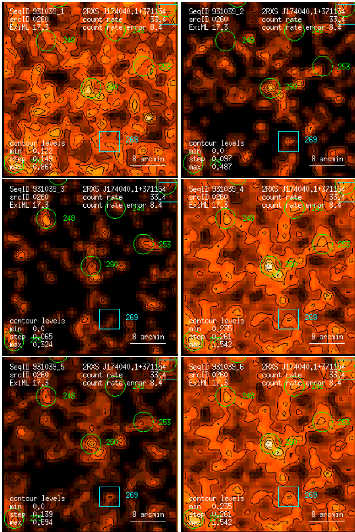
Figure 260: RASS 931039: detection 0260: band rate images, Gaussian filter: (1) PSPC channels 11 – 41, (2) 52 – 90, (3) 91 – 201, (4) 11 – 235, (5) 52 – 201, (6) 11 – 201. Broad band rates in counts/ks. Band rate contour levels in counts/ks/arcmin 2 .
