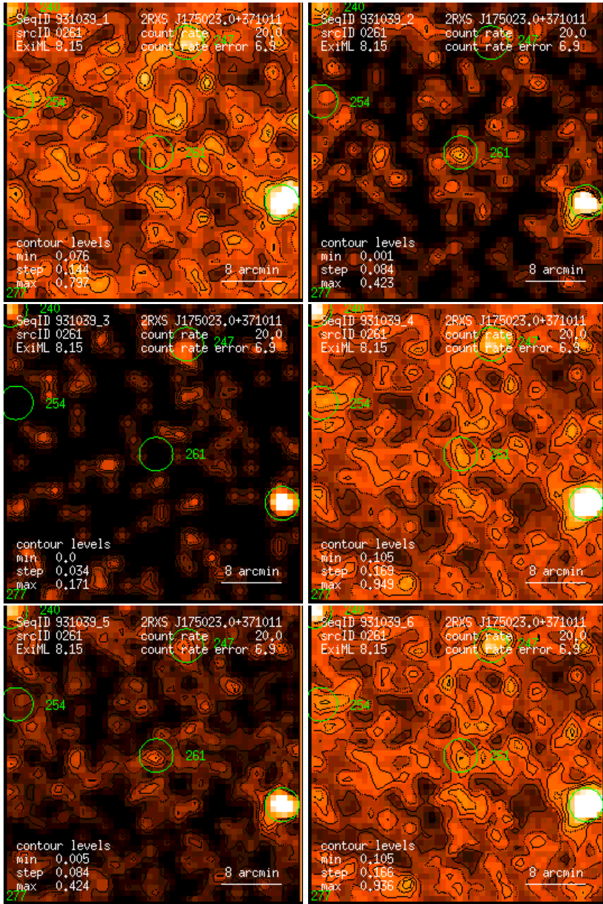
Figure 261: RASS 931039: detection 0261: band rate images, Gaussian filter: (1) PSPC channels 11 – 41, (2) 52 – 90, (3) 91 – 201, (4) 11 – 235, (5) 52 – 201, (6) 11 – 201. Broad band rates in counts/ks. Band rate contour levels in counts/ks/arcmin 2 .
