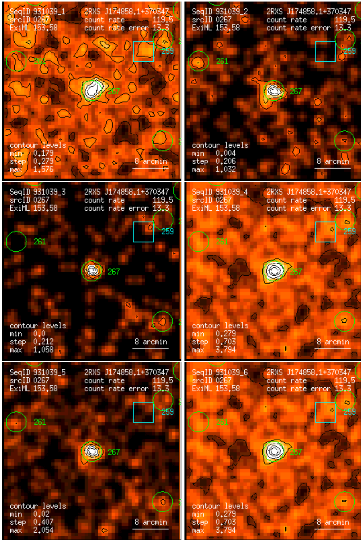
Figure 267: RASS 931039: detection 0267: band rate images, Gaussian filter: (1) PSPC channels 11 – 41, (2) 52 – 90, (3) 91 – 201, (4) 11 – 235, (5) 52 – 201, (6) 11 – 201. Broad band rates in counts/ks. Band rate contour levels in counts/ks/arcmin 2 .
