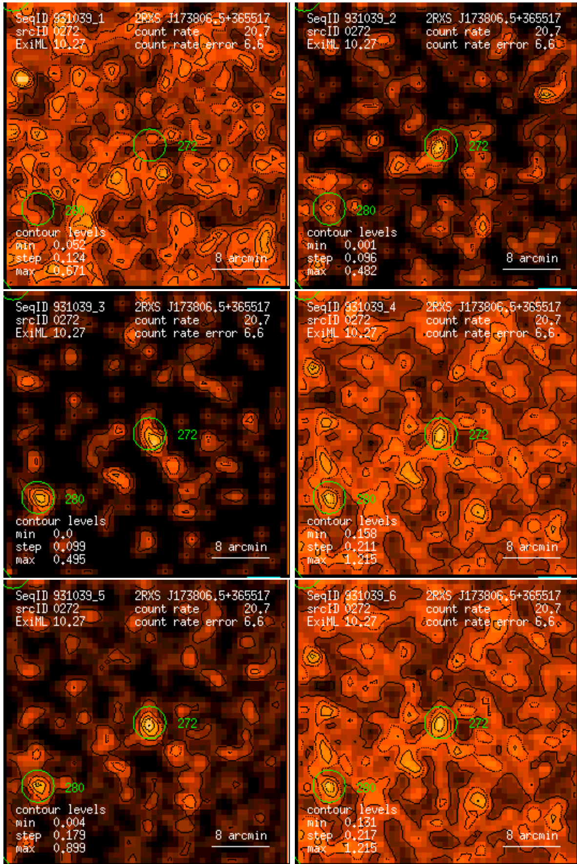
Figure 272: RASS 931039: detection 0272: band rate images, Gaussian filter: (1) PSPC channels 11 – 41, (2) 52 – 90, (3) 91 – 201, (4) 11 – 235, (5) 52 – 201, (6) 11 – 201. Broad band rates in counts/ks. Band rate contour levels in counts/ks/arcmin 2 .
