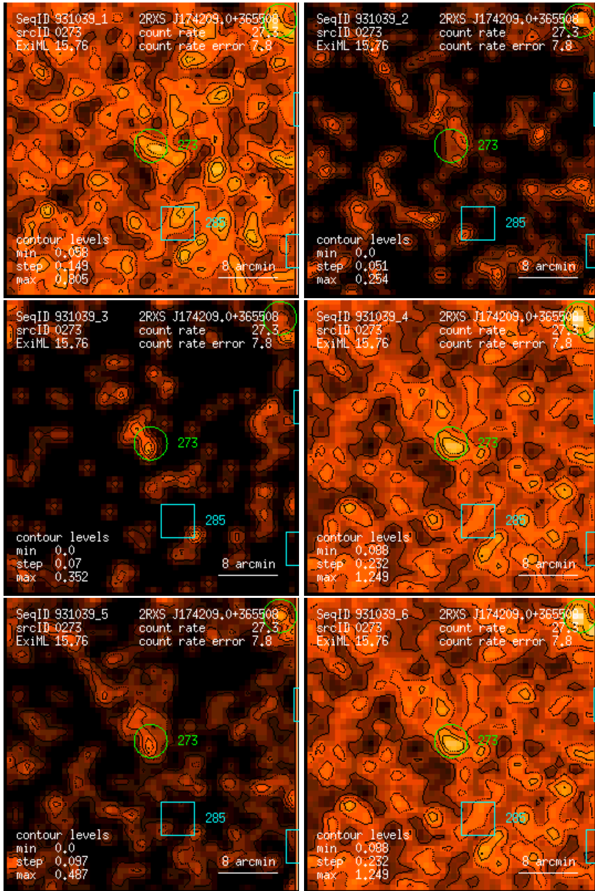
Figure 273: RASS 931039: detection 0273: band rate images, Gaussian filter: (1) PSPC channels 11 – 41, (2) 52 – 90, (3) 91 – 201, (4) 11 – 235, (5) 52 – 201, (6) 11 – 201. Broad band rates in counts/ks. Band rate contour levels in counts/ks/arcmin 2 .
