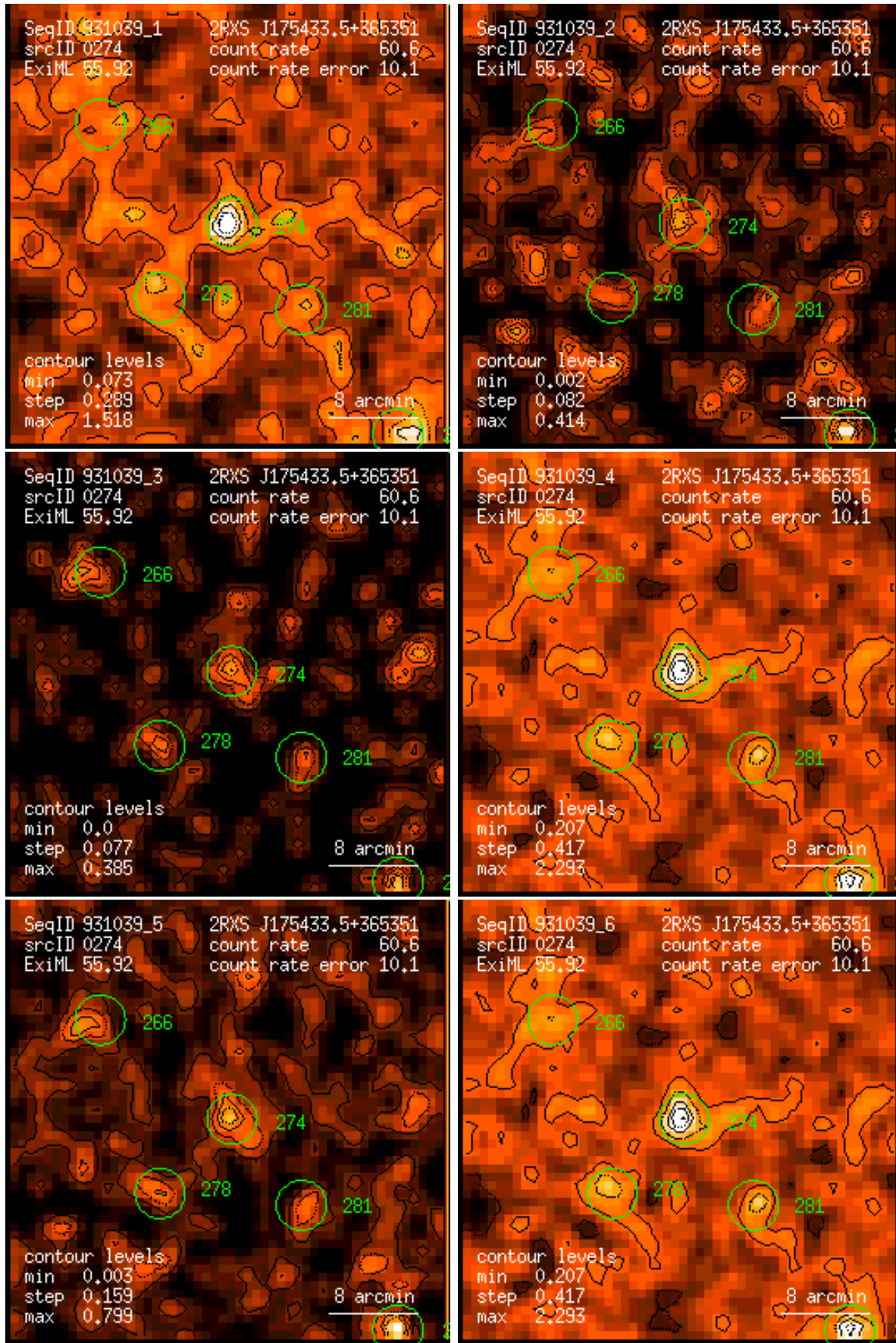
Figure 274: RASS 931039: detection 0274: band rate images, Gaussian filter: (1) PSPPC channels 11 – 41, (2) 52 – 90, (3) 91 – 201, (4) 11 – 235, (5) 52 – 201, (6) 11 – 201. Broad band rates in counts/ks. Band rate contour levels in counts/ks/arcmin 2 .
