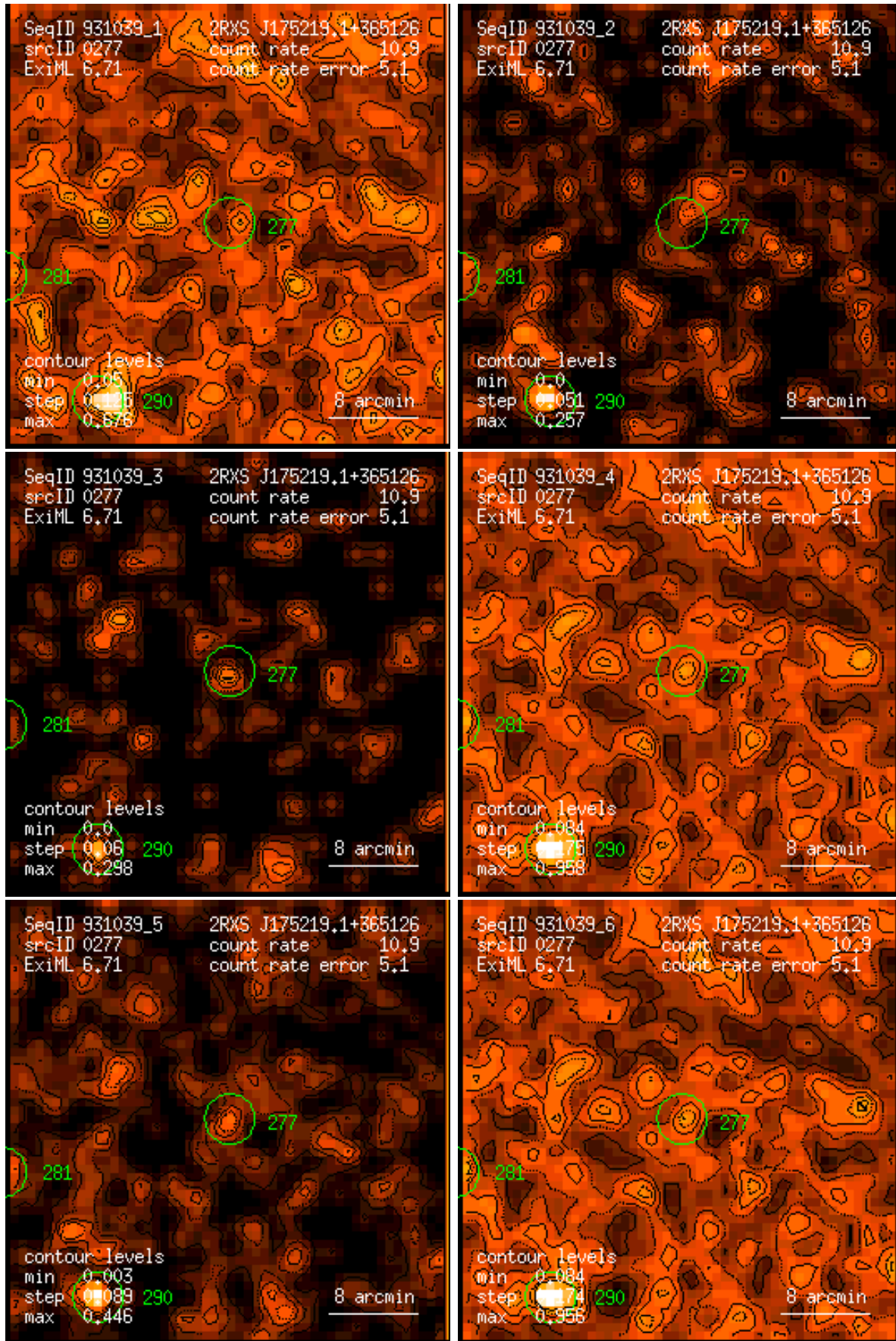
Figure 277: RASS 931039: detection 0277: band rate images, Gaussian filter: (1) PSPC channels 11 – 41, (2) 52 – 90, (3) 91 – 201, (4) 11 – 235, (5) 52 – 201, (6) 11 – 201. Broad band rates in counts/ks. Band rate contour levels in counts/ks/arcmin 2 .
