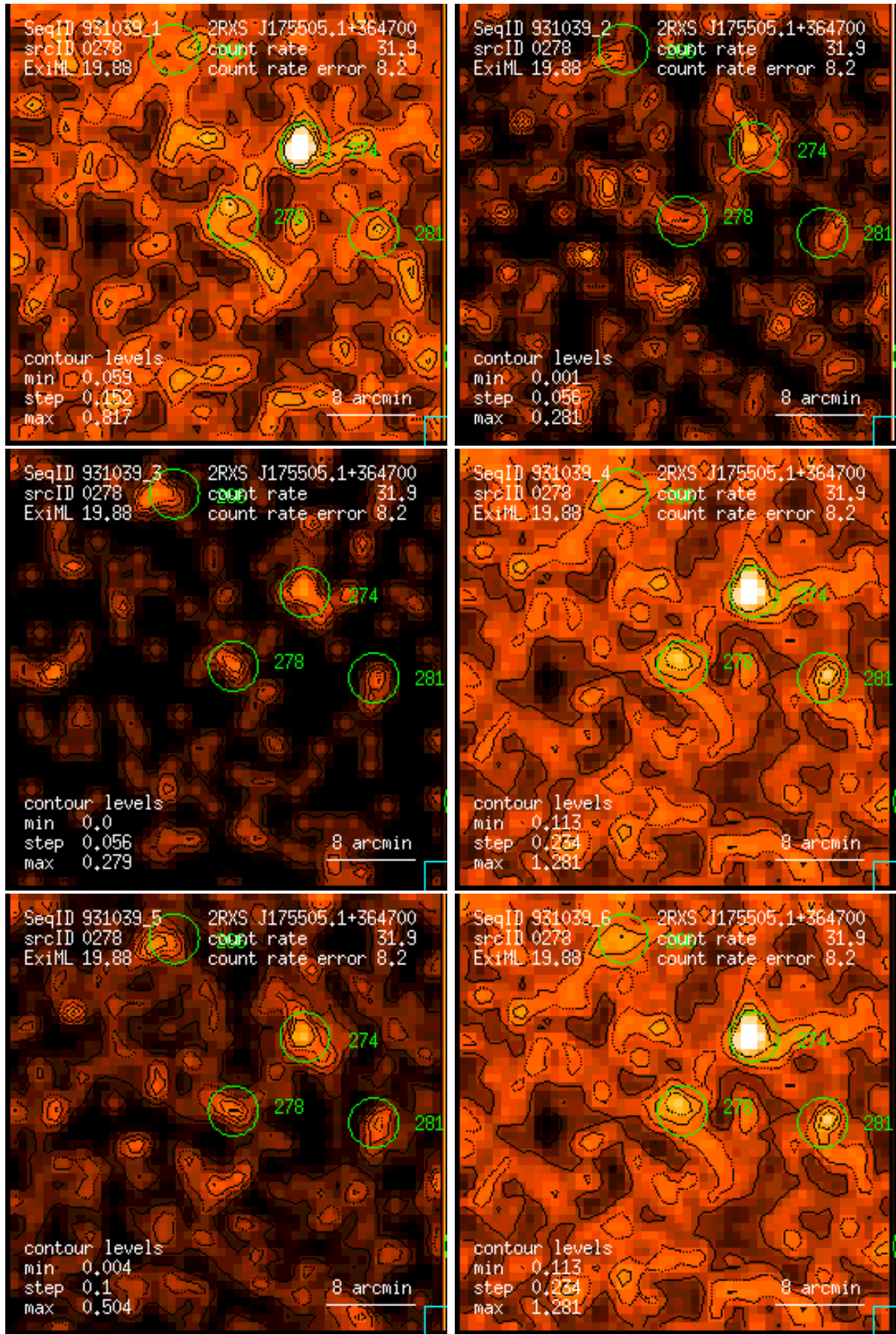
Figure 278: RASS 931039: detection 0278: band rate images, Gaussian filter: (1) PSPC channels 11 – 41, (2) 52 – 90, (3) 91 – 201, (4) 11 – 235, (5) 52 – 201, (6) 11 – 201. Broad band rates in counts/ks. Band rate contour levels in counts/ks/arcmin 2 .
