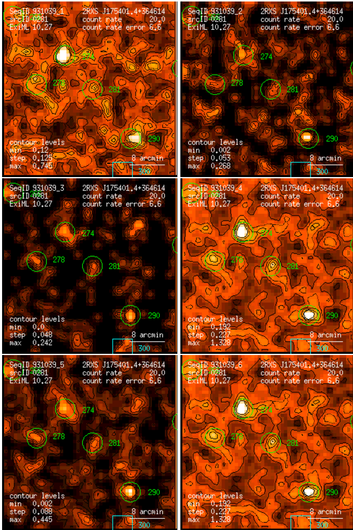
Figure 281: RASS 931039: detection 0281: band rate images, Gaussian filter: (1) PSPC channels 11 – 41, (2) 52 – 90, (3) 91 – 201, (4) 11 – 235, (5) 52 – 201, (6) 11 – 201. Broad band rates in counts/ks. Band rate contour levels in counts/ks/arcmin 2 .
