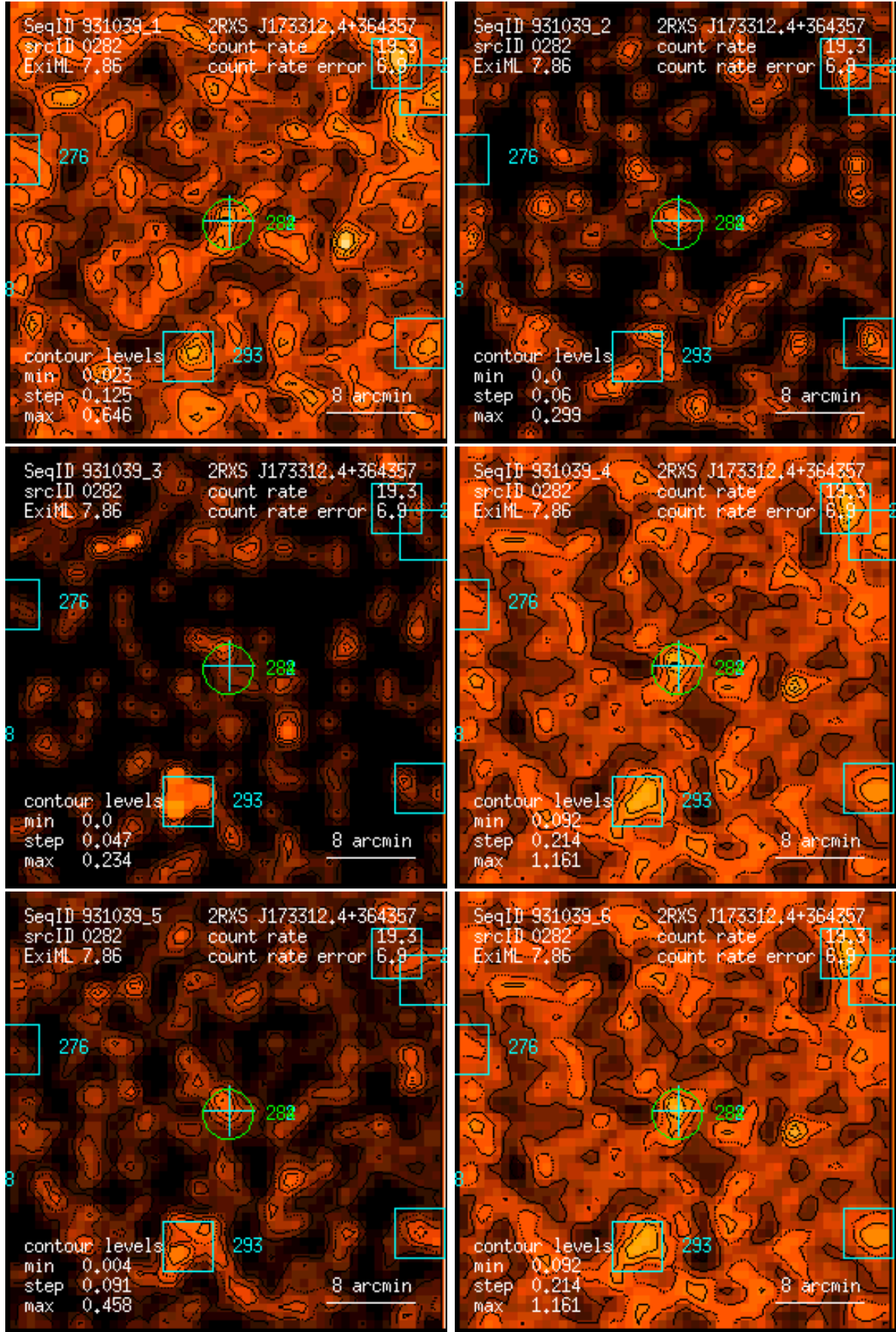
Figure 282: RASS 931039: detection 0282: band rate images, Gaussian filter: (1) PSPC channels 11 – 41, (2) 52 – 90, (3) 91 – 201, (4) 11 – 235, (5) 52 – 201, (6) 11 – 201. Broad band rates in counts/ks. Band rate contour levels in counts/ks/arcmin 2 .
