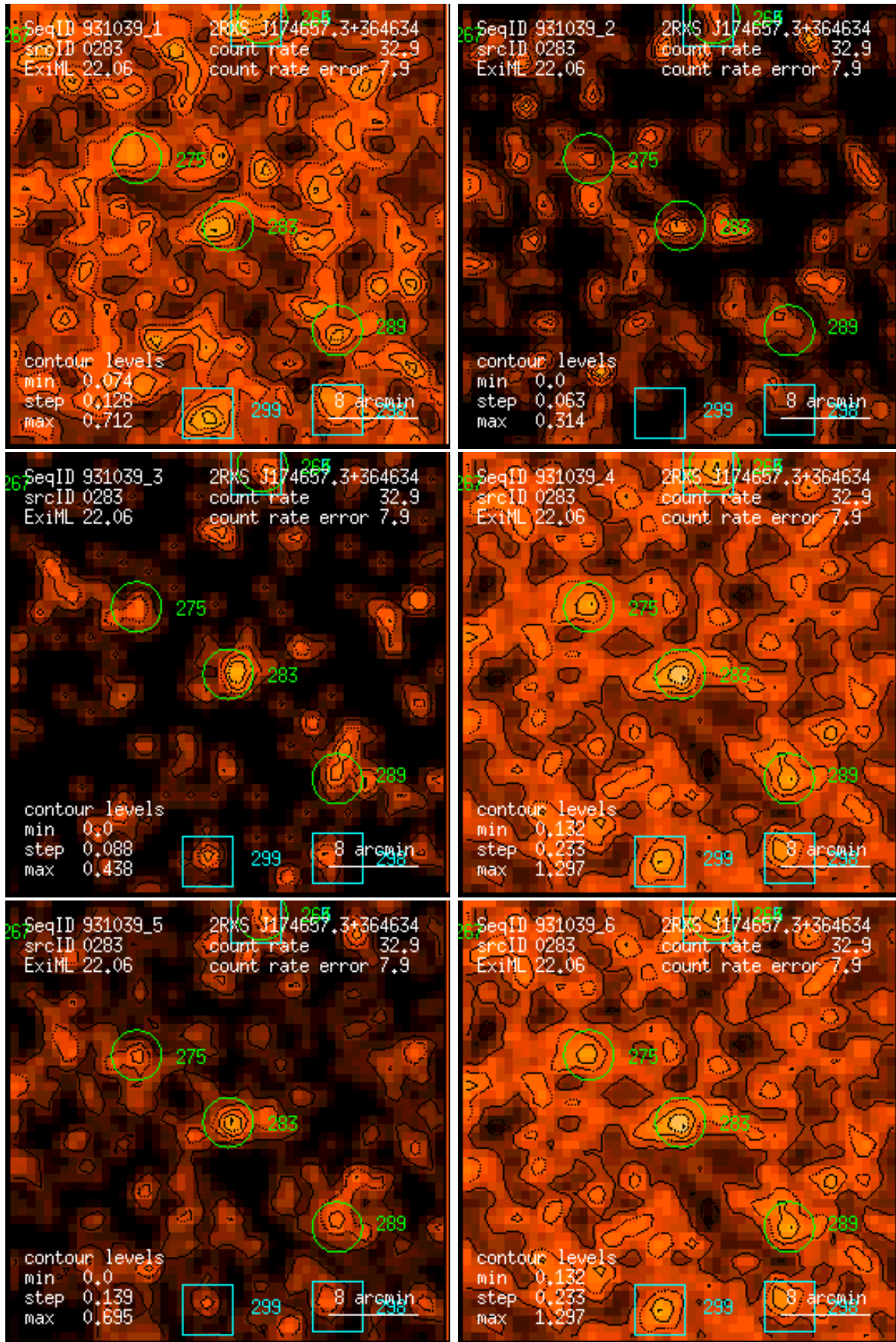
Figure 283: RASS 931039: detection 0283: band rate images, Gaussian filter: (1) PSPC channels 11 – 41, (2) 52 – 90, (3) 91 – 201, (4) 11 – 235, (5) 52 – 201, (6) 11 – 201. Broad band rates in counts/ks. Band rate contour levels in counts/ks/arcmin 2 .
