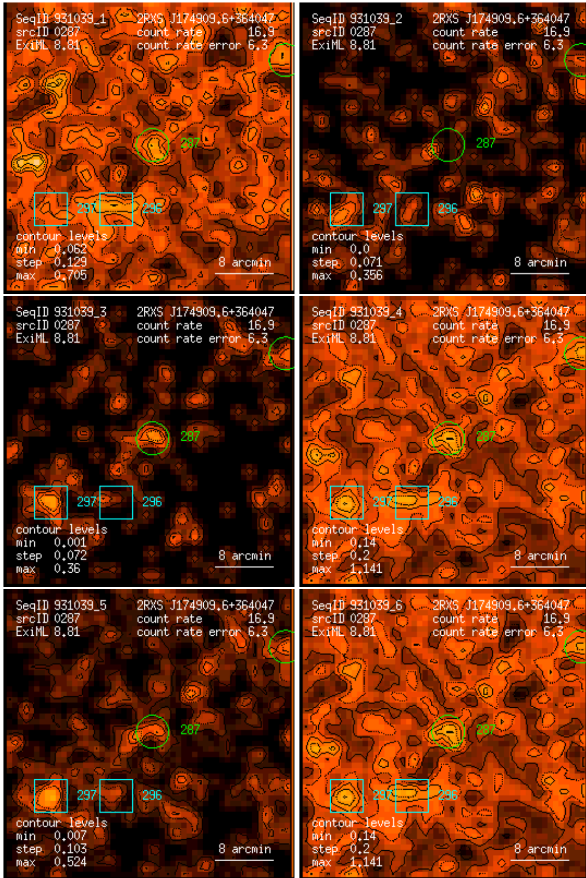
Figure 287: RASS 931039: detection 0287: band rate images, Gaussian filter: (1) PSPC channels 11 – 41, (2) 52 – 90, (3) 91 – 201, (4) 11 – 235, (5) 52 – 201, (6) 11 – 201. Broad band rates in counts/ks. Band rate contour levels in counts/ks/arcmin 2 .
