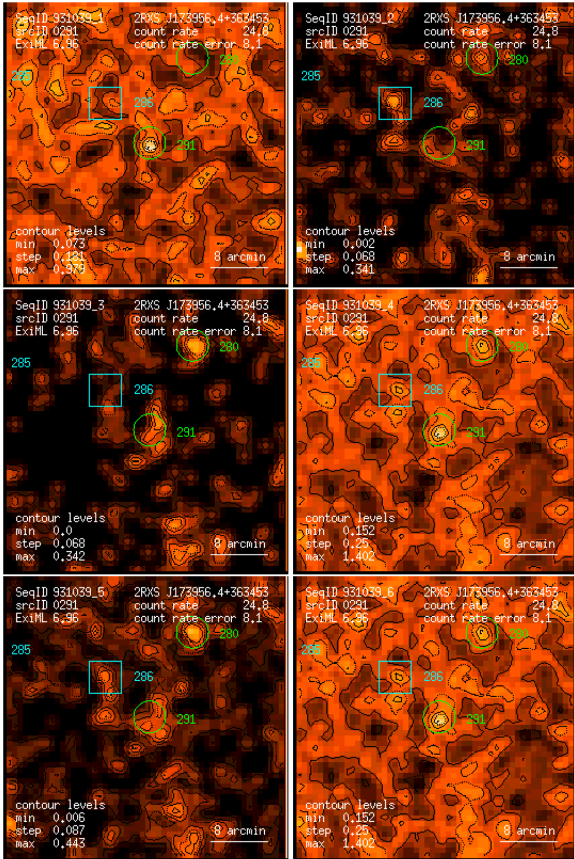
Figure 291: RASS 931039: detection 0291: band rate images, Gaussian filter: (1) PSPC channels 11 – 41, (2) 52 – 90, (3) 91 – 201, (4) 11 – 235, (5) 52 – 201, (6) 11 – 201. Broad band rates in counts/ks. Band rate contour levels in counts/ks/arcmin 2 .
