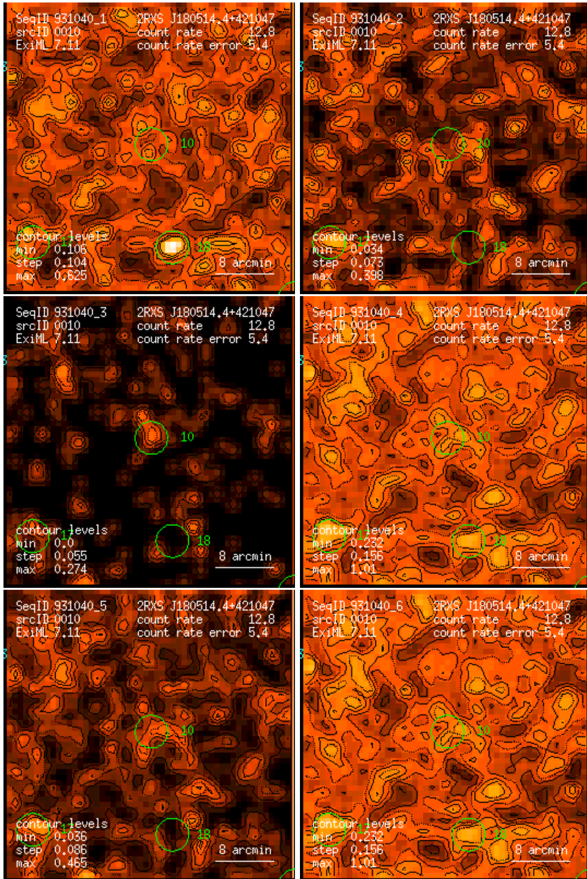
Figure 10: RASS 931040: detection 0010: band rate images, Gaussian filter: (1) PSPC channels 11 – 41, (2) 52 – 90, (3) 91 – 201, (4) 11 – 235, (5) 52 – 201, (6) 11 – 201. Broad band rates in counts/ks. Band rate contour levels in counts/ks/arcmin 2 .
