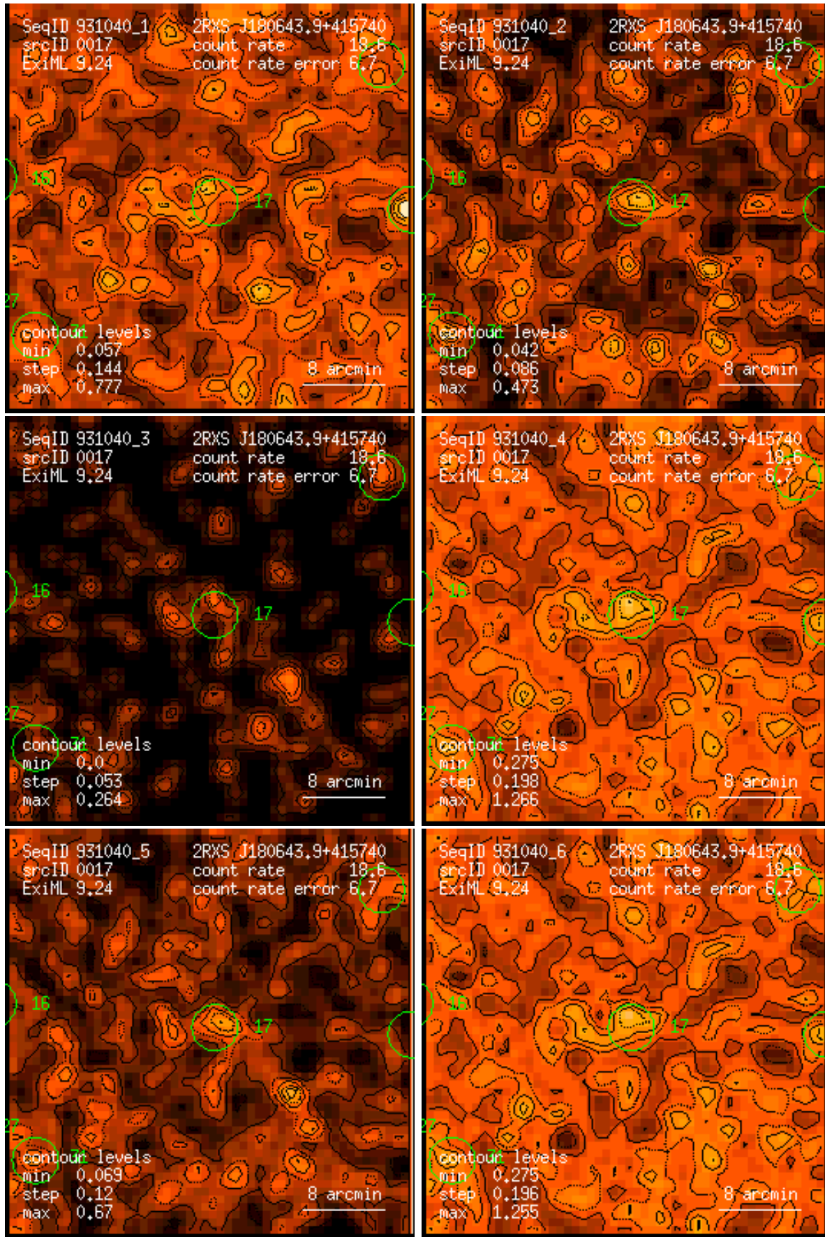
Figure 17: RASS 931040: detection 0017: band rate images, Gaussian filter: (1) PSPC channels 11 – 41, (2) 52 – 90, (3) 91 – 201, (4) 11 – 235, (5) 52 – 201, (6) 11 – 201. Broad band rates in counts/ks. Band rate contour levels in counts/ks/arcmin 2 .
