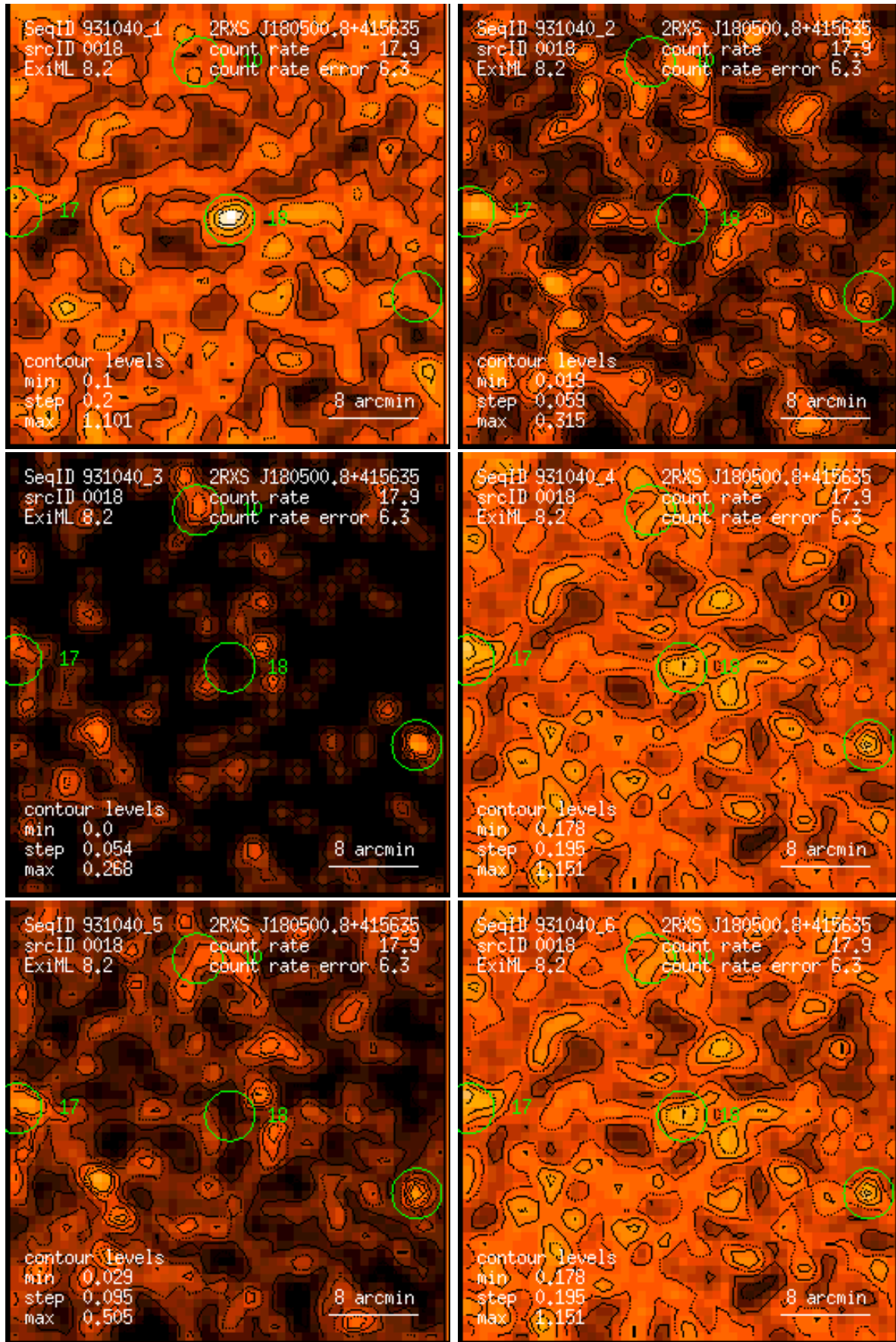
Figure 18: RASS 931040: detection 0018: band rate images, Gaussian filter: (1) PSPC channels 11 – 41, (2) 52 – 90, (3) 91 – 201, (4) 11 – 235, (5) 52 – 201, (6) 11 – 201. Broad band rates in counts/ks. Band rate contour levels in counts/ks/arcmin 2 .
