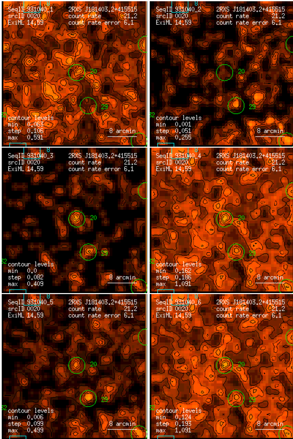
Figure 20: RASS 931040: detection 0020: band rate images, Gaussian filter: (1) PSPC channels 11 – 41, (2) 52 – 90, (3) 91 – 201, (4) 11 – 235, (5) 52 – 201, (6) 11 – 201. Broad band rates in counts/ks. Band rate contour levels in counts/ks/arcmin 2 .
