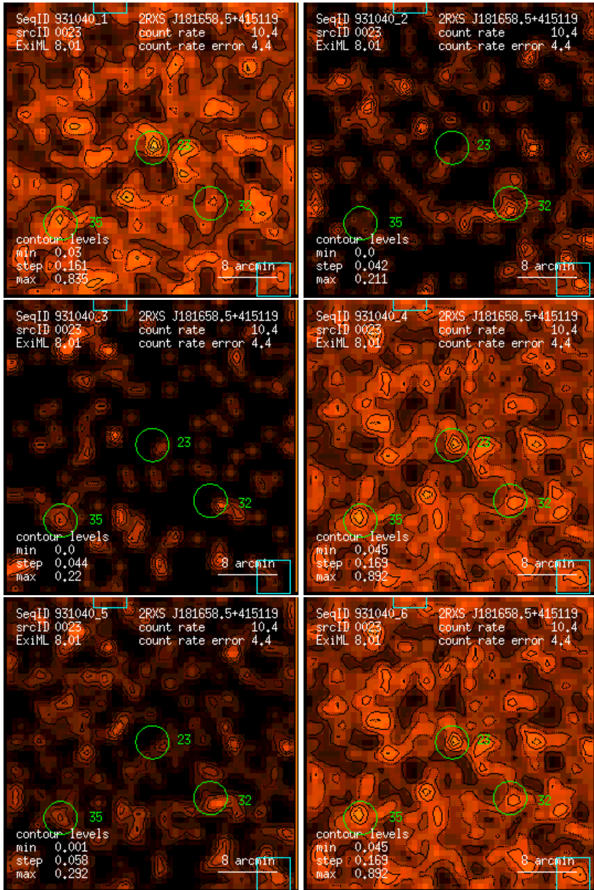
Figure 23: RASS 931040: detection 0023: band rate images, Gaussian filter: (1) PSPC channels 11 – 41, (2) 52 – 90, (3) 91 – 201, (4) 11 – 235, (5) 52 – 201, (6) 11 – 201. Broad band rates in counts/ks. Band rate contour levels in counts/ks/arcmin 2 .
