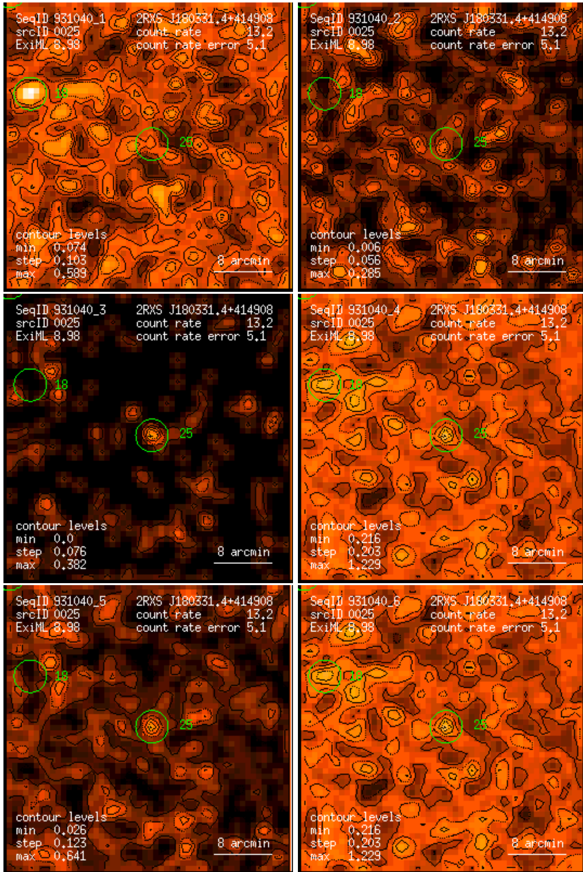
Figure 25: RASS 931040: detection 0025: band rate images, Gaussian filter: (1) PSPC channels 11 – 41, (2) 52 – 90, (3) 91 – 201, (4) 11 – 235, (5) 52 – 201, (6) 11 – 201. Broad band rates in counts/ks. Band rate contour levels in counts/ks/arcmin 2 .
