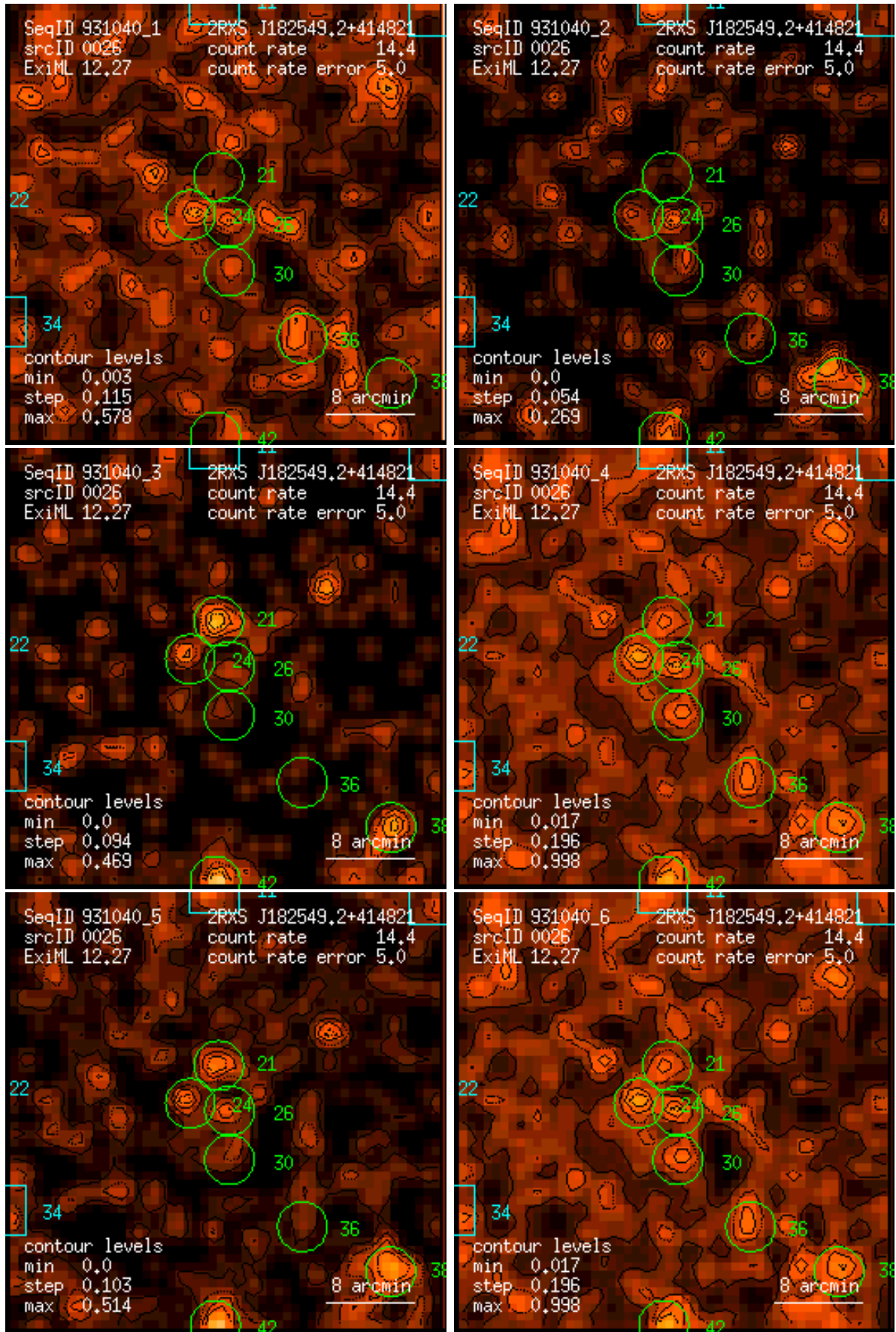
Figure 26: RASS 931040: detection 0026: band rate images, Gaussian filter: (1) PSPC channels 11 – 41, (2) 52 – 90, (3) 91 – 201, (4) 11 – 235, (5) 52 – 201, (6) 11 – 201. Broad band rates in counts/ks. Band rate contour levels in counts/ks/arcmin 2 .
