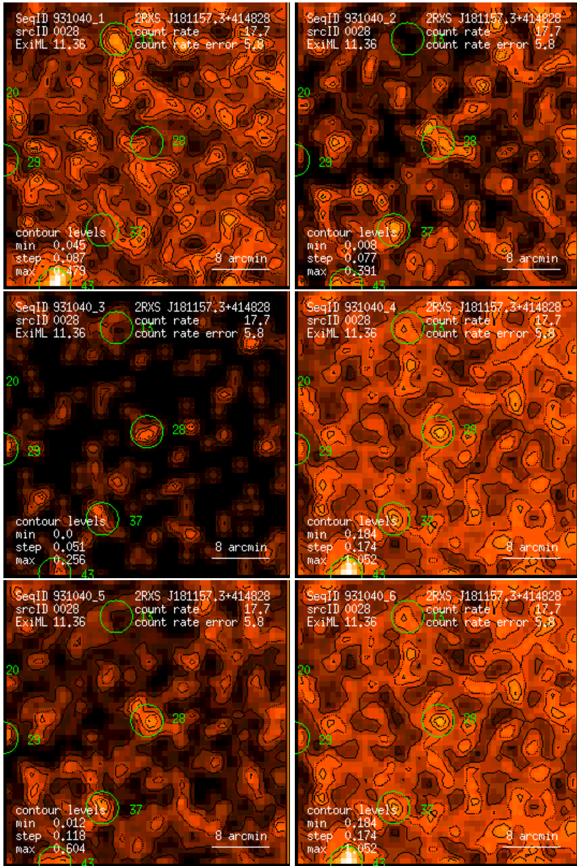
Figure 28: RASS 931040: detection 0028: band rate images, Gaussian filter: (1) PSPC channels 11 – 41, (2) 52 – 90, (3) 91 – 201, (4) 11 – 235, (5) 52 – 201, (6) 11 – 201. Broad band rates in counts/ks. Band rate contour levels in counts/ks/arcmin 2 .
