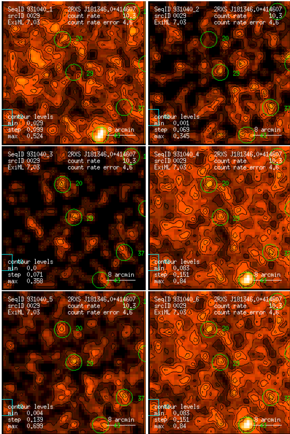
Figure 29: RASS 931040: detection 0029: band rate images, Gaussian filter: (1) PSPC channels 11 – 41, (2) 52 – 90, (3) 91 – 201, (4) 11 – 235, (5) 52 – 201, (6) 11 – 201. Broad band rates in counts/ks. Band rate contour levels in counts/ks/arcmin 2 .
