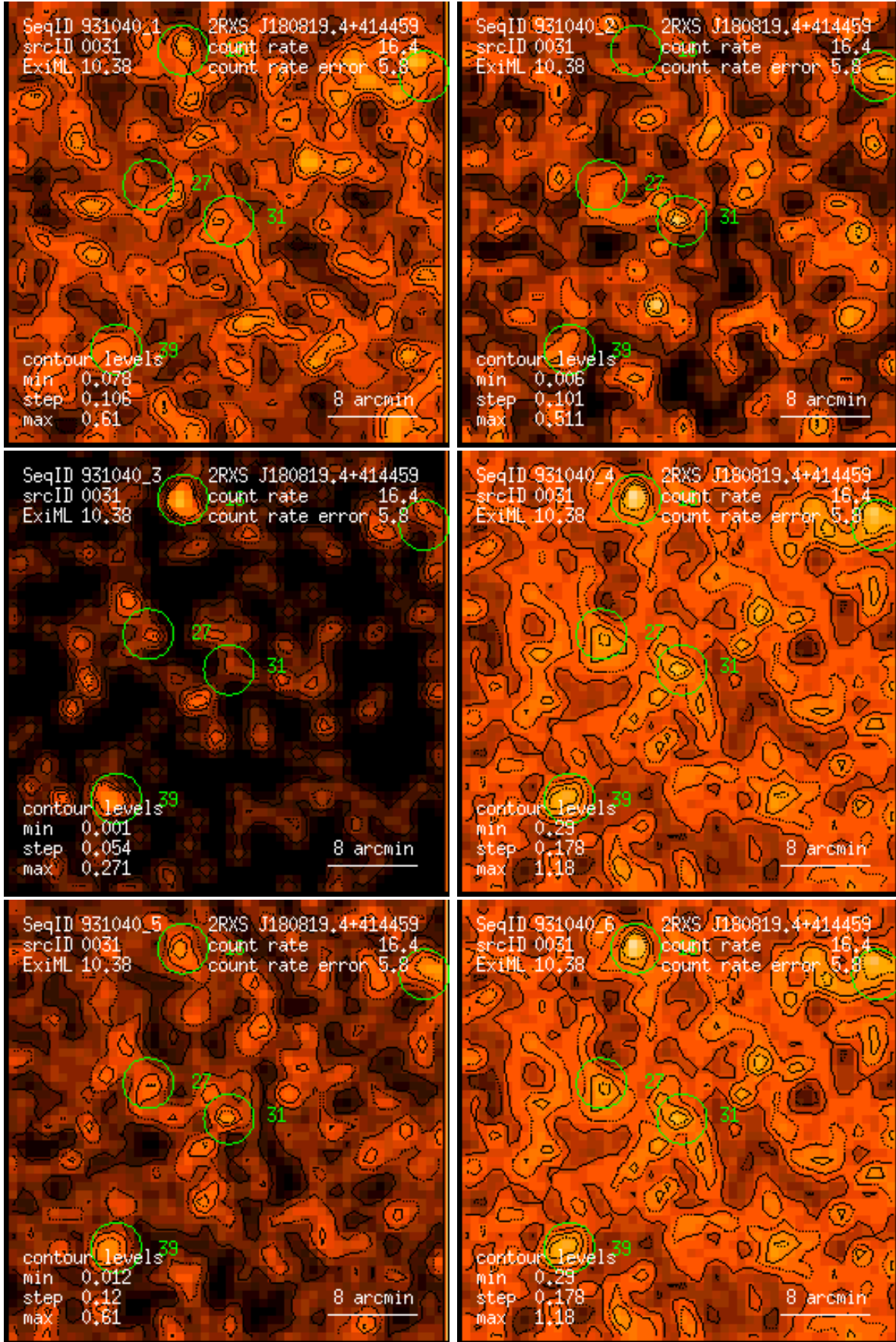
Figure 31: RASS 931040: detection 0031: band rate images, Gaussian filter: (1) PSPC channels 11 – 41, (2) 52 – 90, (3) 91 – 201, (4) 11 – 235, (5) 52 – 201, (6) 11 – 201. Broad band rates in counts/ks. Band rate contour levels in counts/ks/arcmin 2 .
