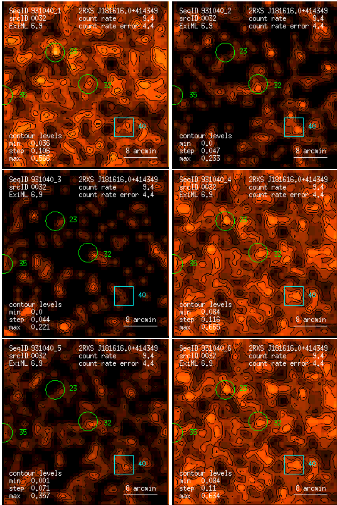
Figure 32: RASS 931040: detection 0032: band rate images, Gaussian filter: (1) PSPC channels 11 – 41, (2) 52 – 90, (3) 91 – 201, (4) 11 – 235, (5) 52 – 201, (6) 11 – 201. Broad band rates in counts/ks. Band rate contour levels in counts/ks/arcmin 2 .
