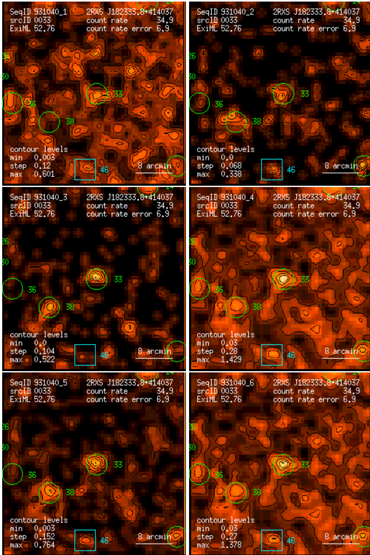
Figure 33: RASS 931040: detection 0033: band rate images, Gaussian filter: (1) PSPC channels 11 – 41, (2) 52 – 90, (3) 91 – 201, (4) 11 – 235, (5) 52 – 201, (6) 11 – 201. Broad band rates in counts/ks. Band rate contour levels in counts/ks/arcmin 2 .
