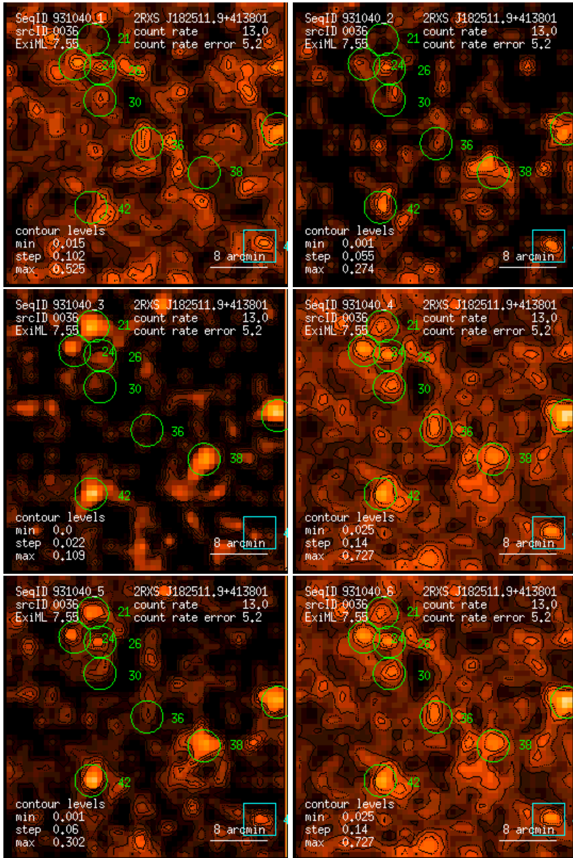
Figure 36: RASS 931040: detection 0036: band rate images, Gaussian filter: (1) PSPC channels 11 – 41, (2) 52 – 90, (3) 91 – 201, (4) 11 – 235, (5) 52 – 201, (6) 11 – 201. Broad band rates in counts/ks. Band rate contour levels in counts/ks/arcmin 2 .
