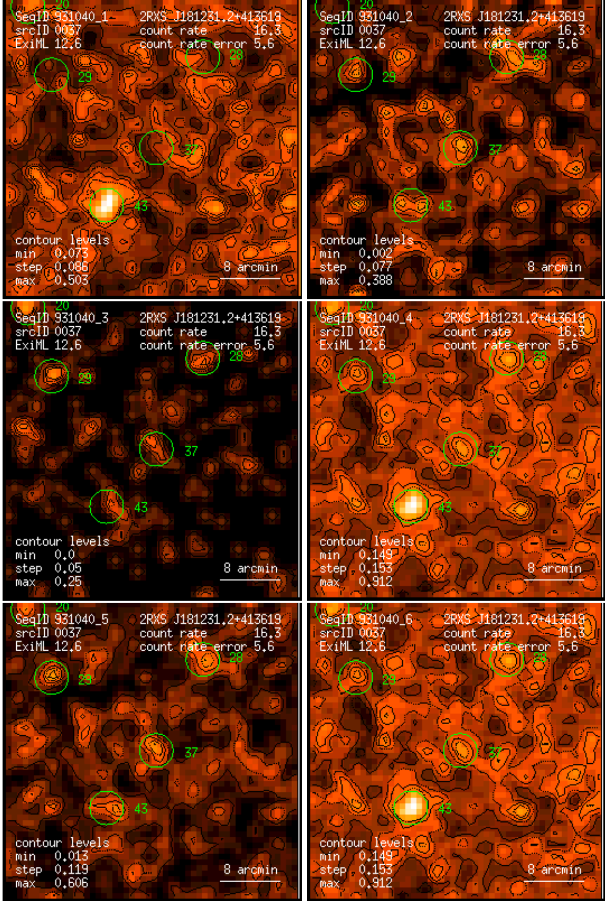
Figure 37: RASS 931040: detection 0037: band rate images, Gaussian filter: (1) PSPC channels 11 – 41, (2) 52 – 90, (3) 91 – 201, (4) 11 – 235, (5) 52 – 201, (6) 11 – 201. Broad band rates in counts/ks. Band rate contour levels in counts/ks/arcmin 2 .
