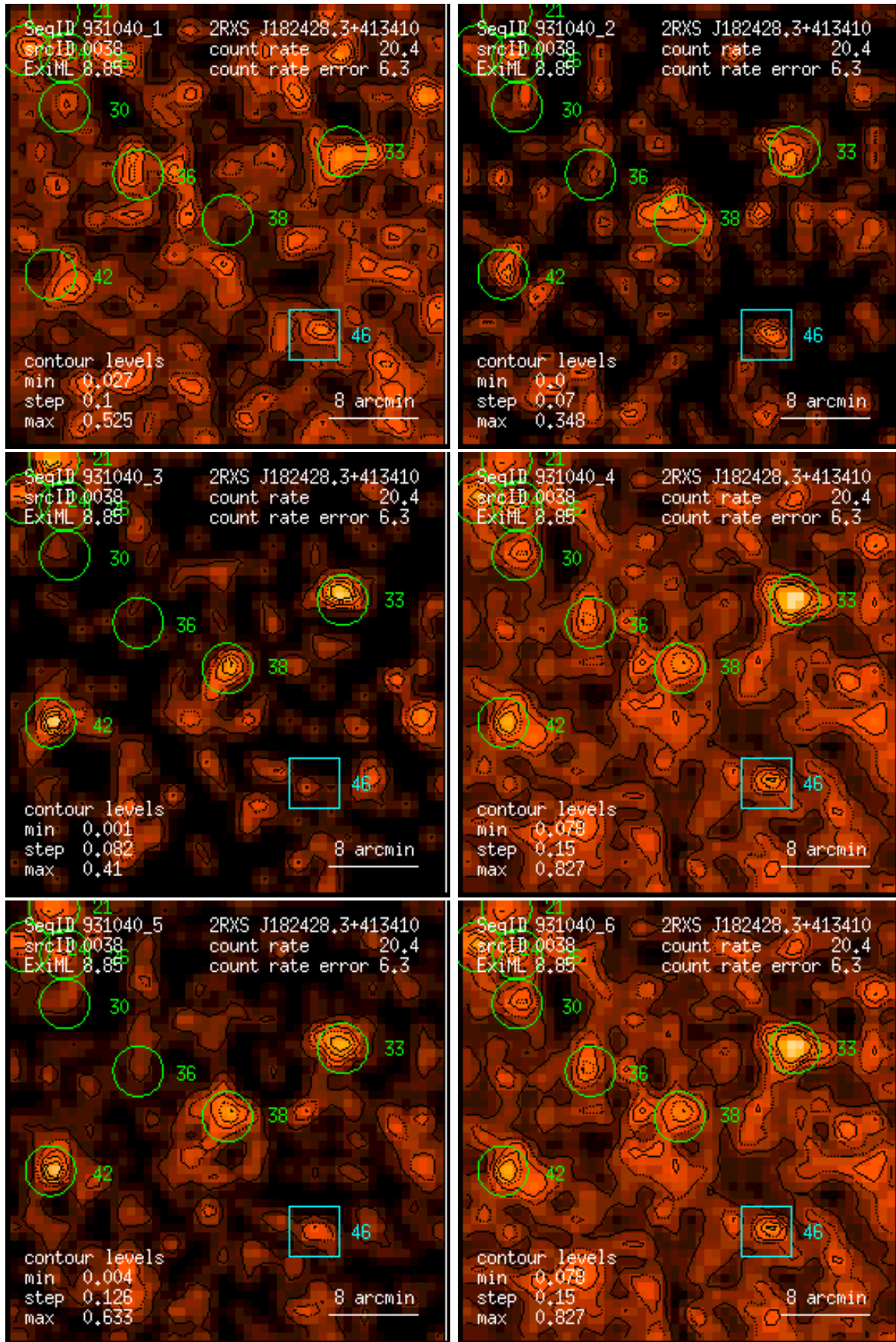
Figure 38: RASS 931040: detection 0038: band rate images, Gaussian filter: (1) PSPC channels 11 – 41, (2) 52 – 90, (3) 91 – 201, (4) 11 – 235, (5) 52 – 201, (6) 11 – 201. Broad band rates in counts/ks. Band rate contour levels in counts/ks/arcmin 2 .
