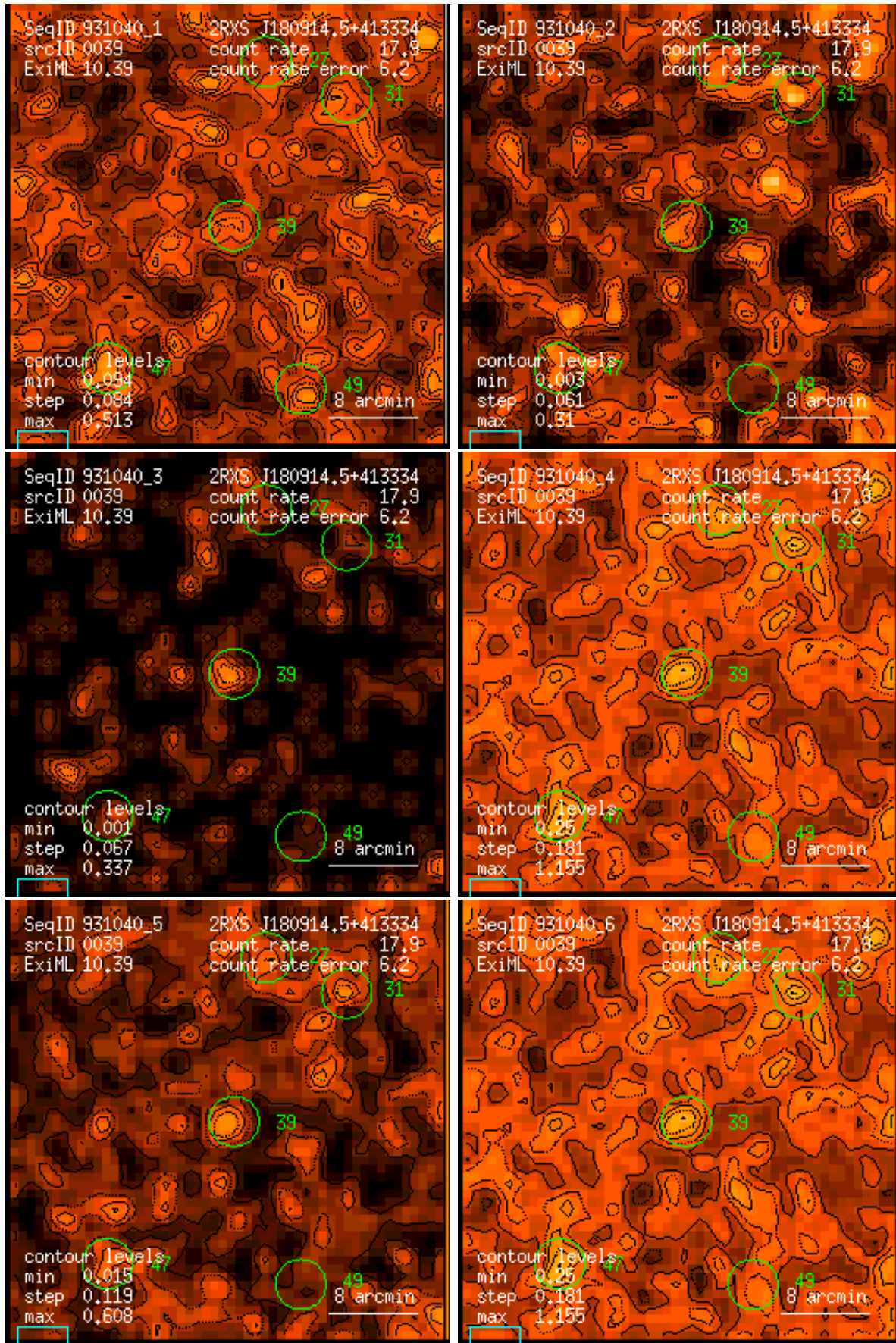
Figure 39: RASS 931040: detection 0039: band rate images, Gaussian filter: (1) PSPC channels 11 – 41, (2) 52 – 90, (3) 91 – 201, (4) 11 – 235, (5) 52 – 201, (6) 11 – 201. Broad band rates in counts/ks. Band rate contour levels in counts/ks/arcmin 2 .
