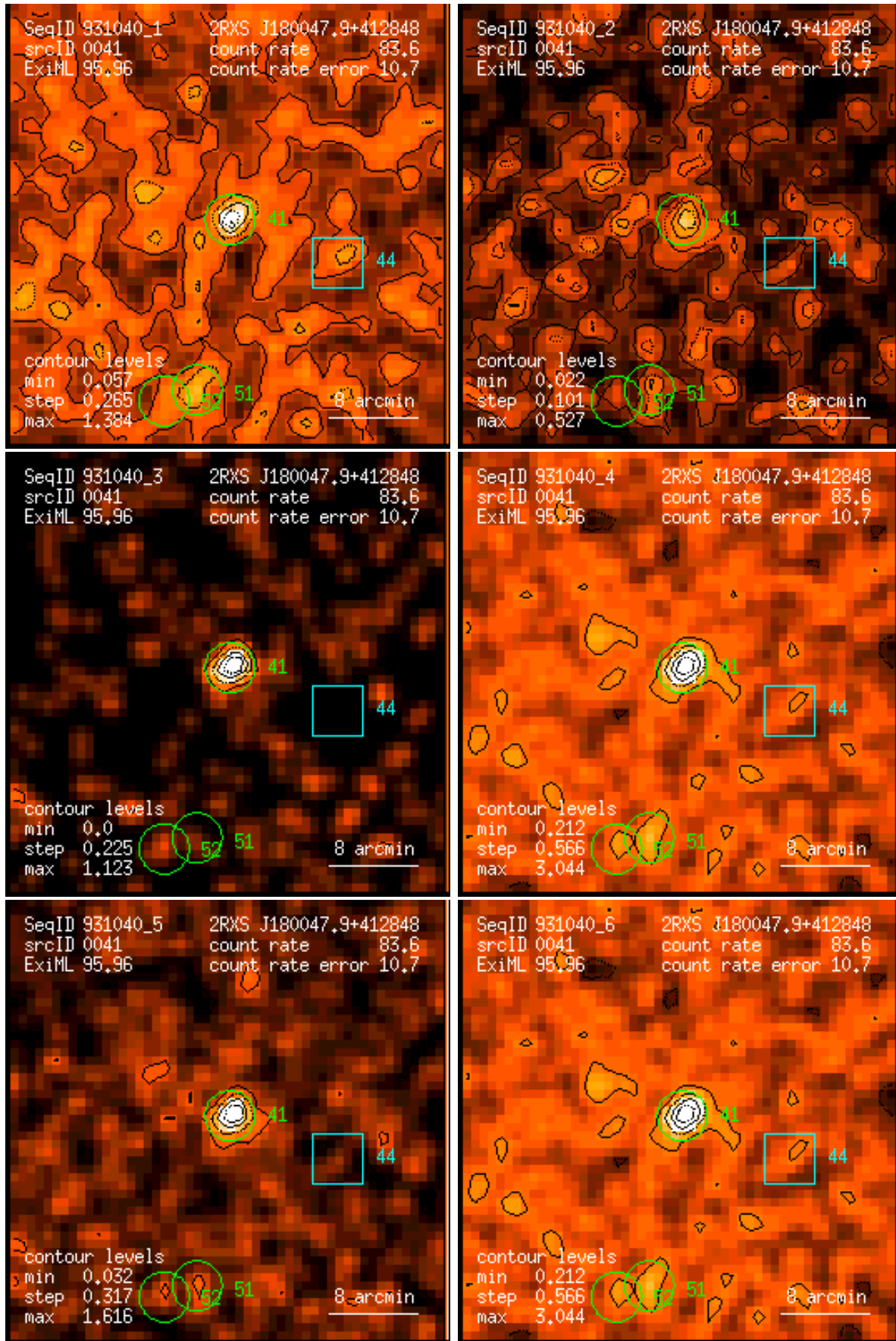
Figure 41: RASS 931040: detection 0041: band rate images, Gaussian filter: (1) PSPC channels 11 – 41, (2) 52 – 90, (3) 91 – 201, (4) 11 – 235, (5) 52 – 201, (6) 11 – 201. Broad band rates in counts/ks. Band rate contour levels in counts/ks/arcmin 2 .
