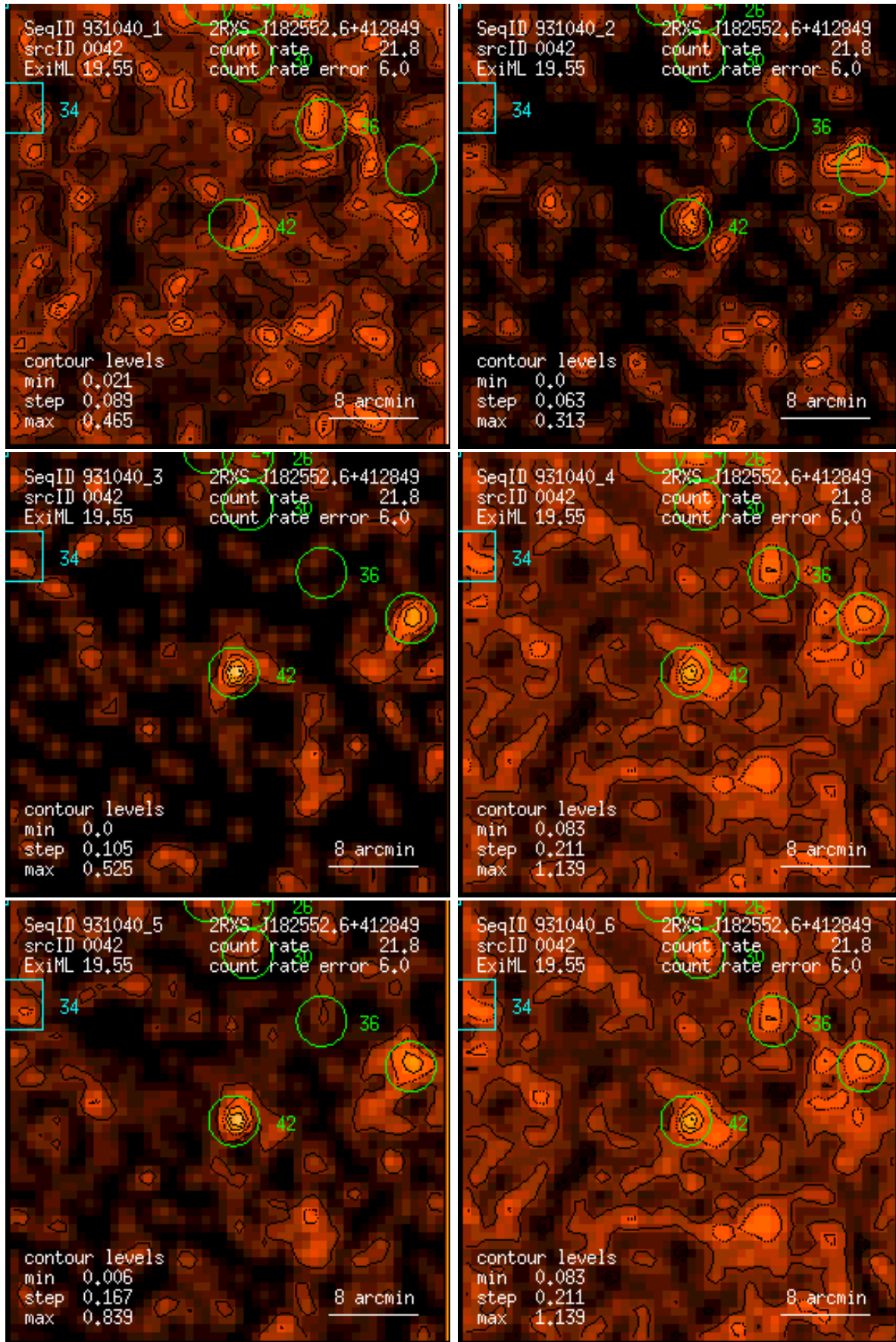
Figure 42: RASS 931040: detection 0042: band rate images, Gaussian filter: (1) PSPC channels 11 – 41, (2) 52 – 90, (3) 91 – 201, (4) 11 – 235, (5) 52 – 201, (6) 11 – 201. Broad band rates in counts/ks. Band rate contour levels in counts/ks/arcmin 2 .
