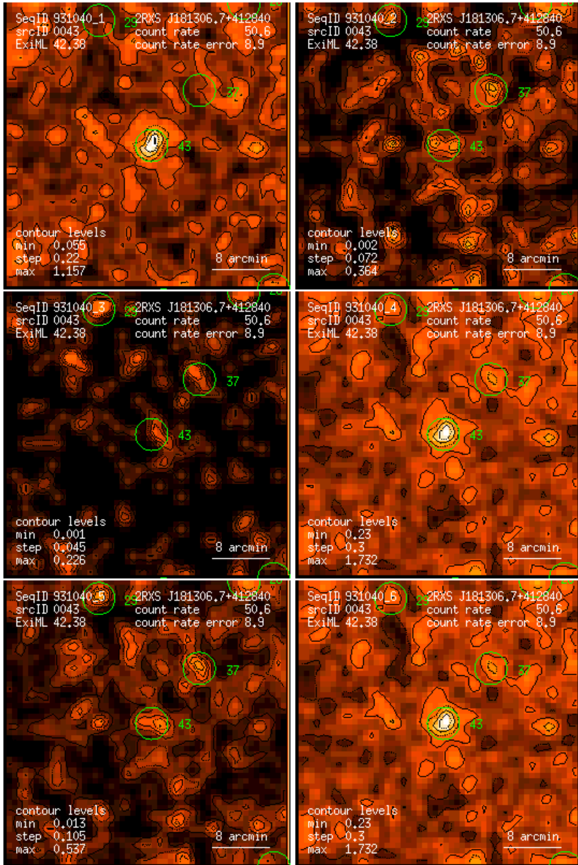
Figure 43: RASS 931040: detection 0043: band rate images, Gaussian filter: (1) PSPC channels 11 – 41, (2) 52 – 90, (3) 91 – 201, (4) 11 – 235, (5) 52 – 201, (6) 11 – 201. Broad band rates in counts/ks. Band rate contour levels in counts/ks/arcmin 2 .
