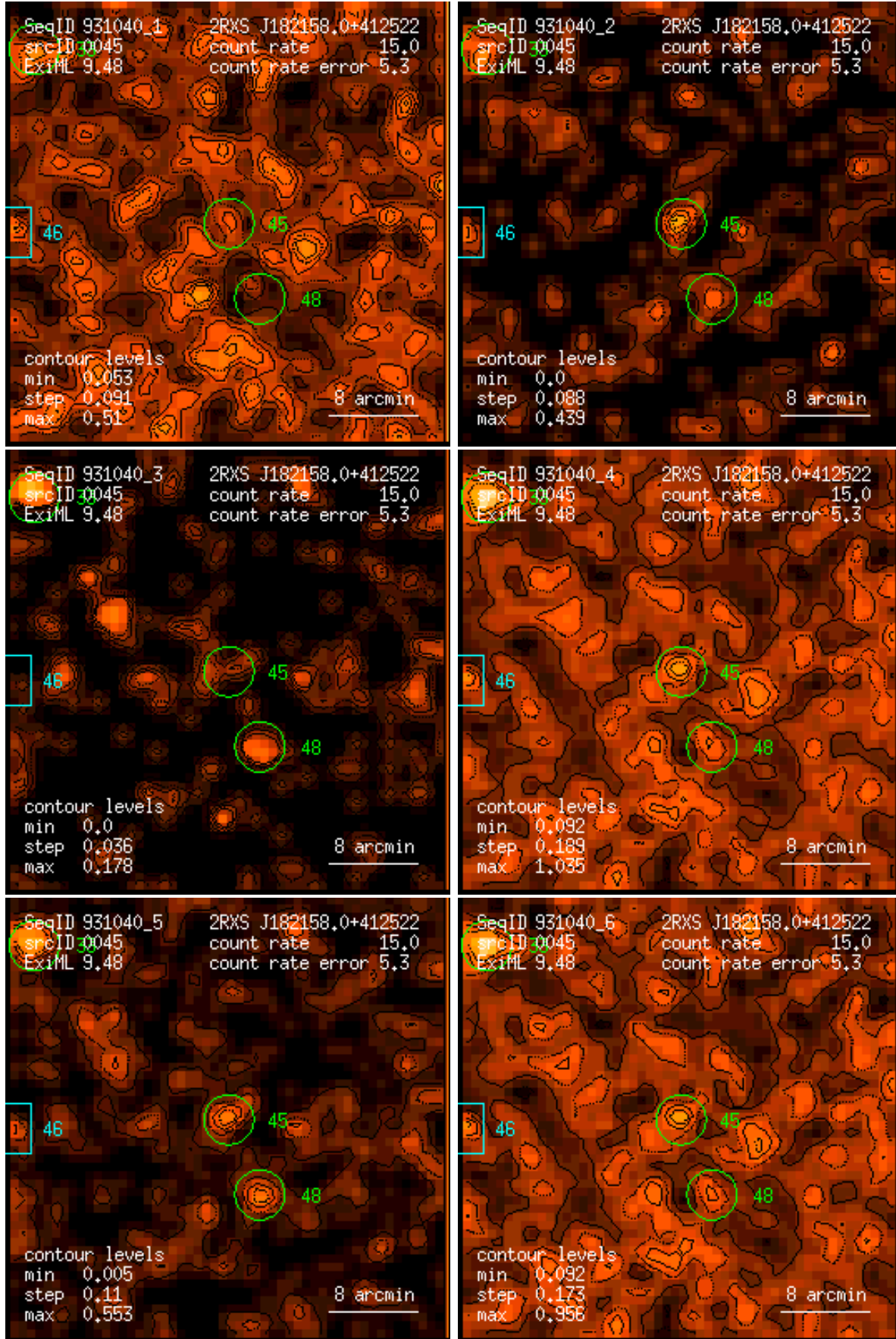
Figure 45: RASS 931040: detection 0045: band rate images, Gaussian filter: (1) PSPC channels 11 – 41, (2) 52 – 90, (3) 91 – 201, (4) 11 – 235, (5) 52 – 201, (6) 11 – 201. Broad band rates in counts/ks. Band rate contour levels in counts/ks/arcmin 2 .
