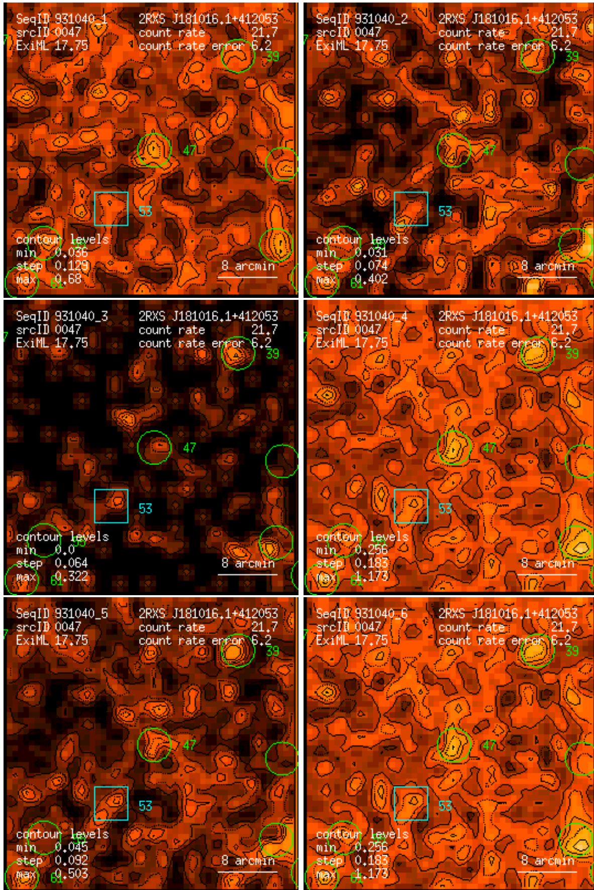
Figure 47: RASS 931040: detection 0047: band rate images, Gaussian filter: (1) PSPC channels 11 – 41, (2) 52 – 90, (3) 91 – 201, (4) 11 – 235, (5) 52 – 201, (6) 11 – 201. Broad band rates in counts/ks. Band rate contour levels in counts/ks/arcmin 2 .
