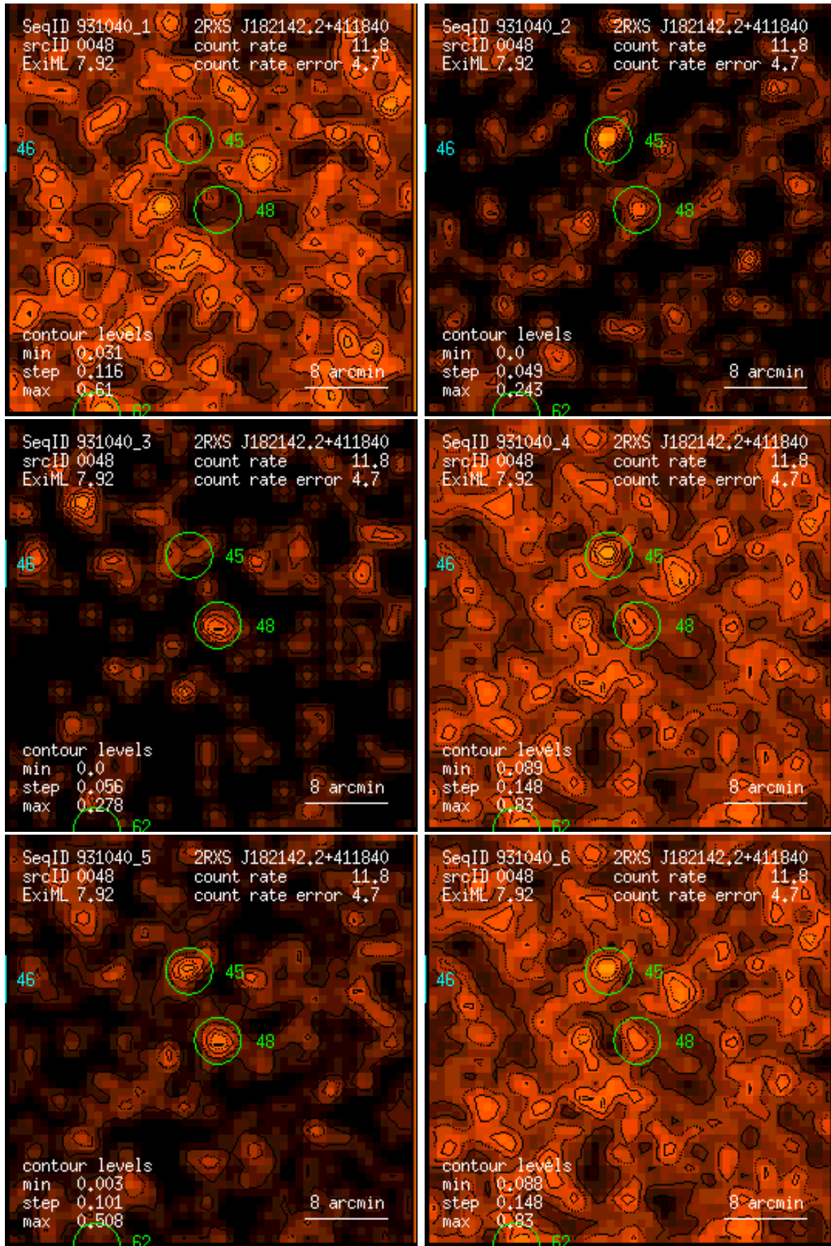
Figure 48: RASS 931040: detection 0048: band rate images, Gaussian filter: (1) PSPC channels 11 – 41, (2) 52 – 90, (3) 91 – 201, (4) 11 – 235, (5) 52 – 201, (6) 11 – 201. Broad band rates in counts/ks. Band rate contour levels in counts/ks/arcmin 2 .
