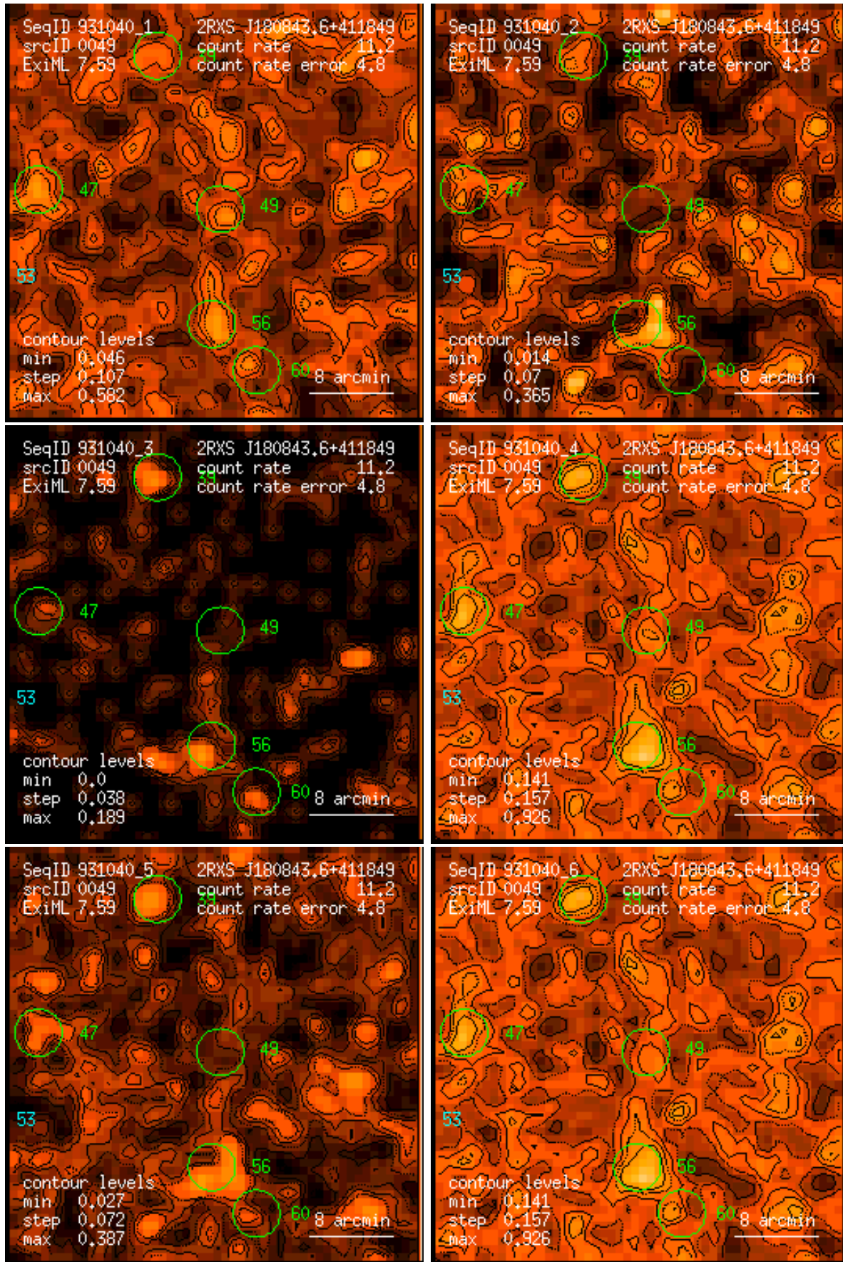
Figure 49: RASS 931040: detection 0049: band rate images, Gaussian filter: (1) PSPC channels 11 – 41, (2) 52 – 90, (3) 91 – 201, (4) 11 – 235, (5) 52 – 201, (6) 11 – 201. Broad band rates in counts/ks. Band rate contour levels in counts/ks/arcmin 2 .
