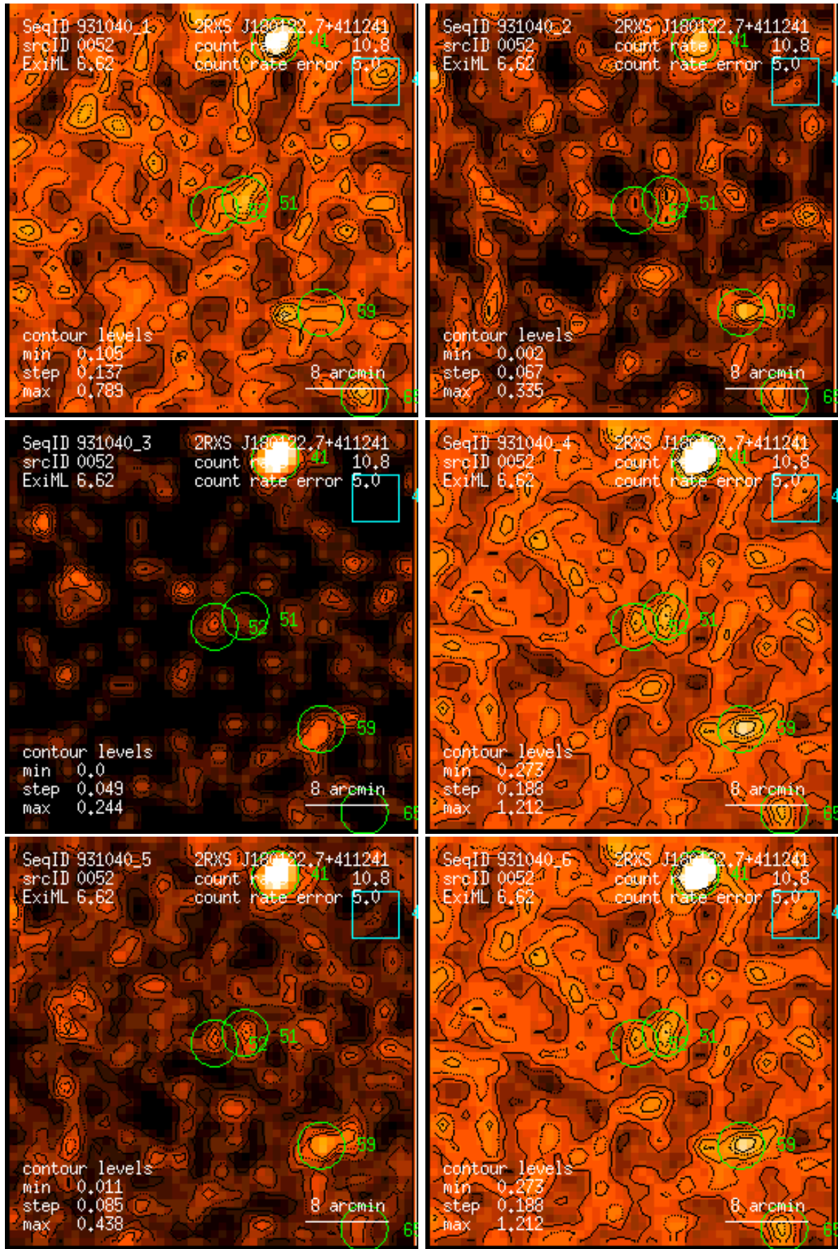
Figure 52: RASS 931040: detection 0052: band rate images, Gaussian filter: (1) PSPC channels 11 – 41, (2) 52 – 90, (3) 91 – 201, (4) 11 – 235, (5) 52 – 201, (6) 11 – 201. Broad band rates in counts/ks. Band rate contour levels in counts/ks/arcmin 2 .
