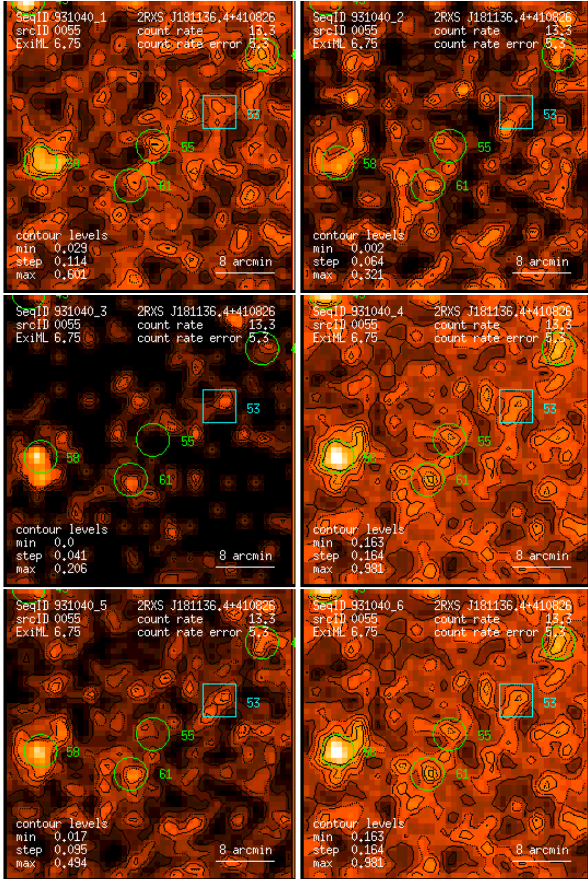
Figure 55: RASS 931040: detection 0055: band rate images, Gaussian filter: (1) PSPC channels 11 – 41, (2) 52 – 90, (3) 91 – 201, (4) 11 – 235, (5) 52 – 201, (6) 11 – 201. Broad band rates in counts/ks. Band rate contour levels in counts/ks/arcmin 2 .
