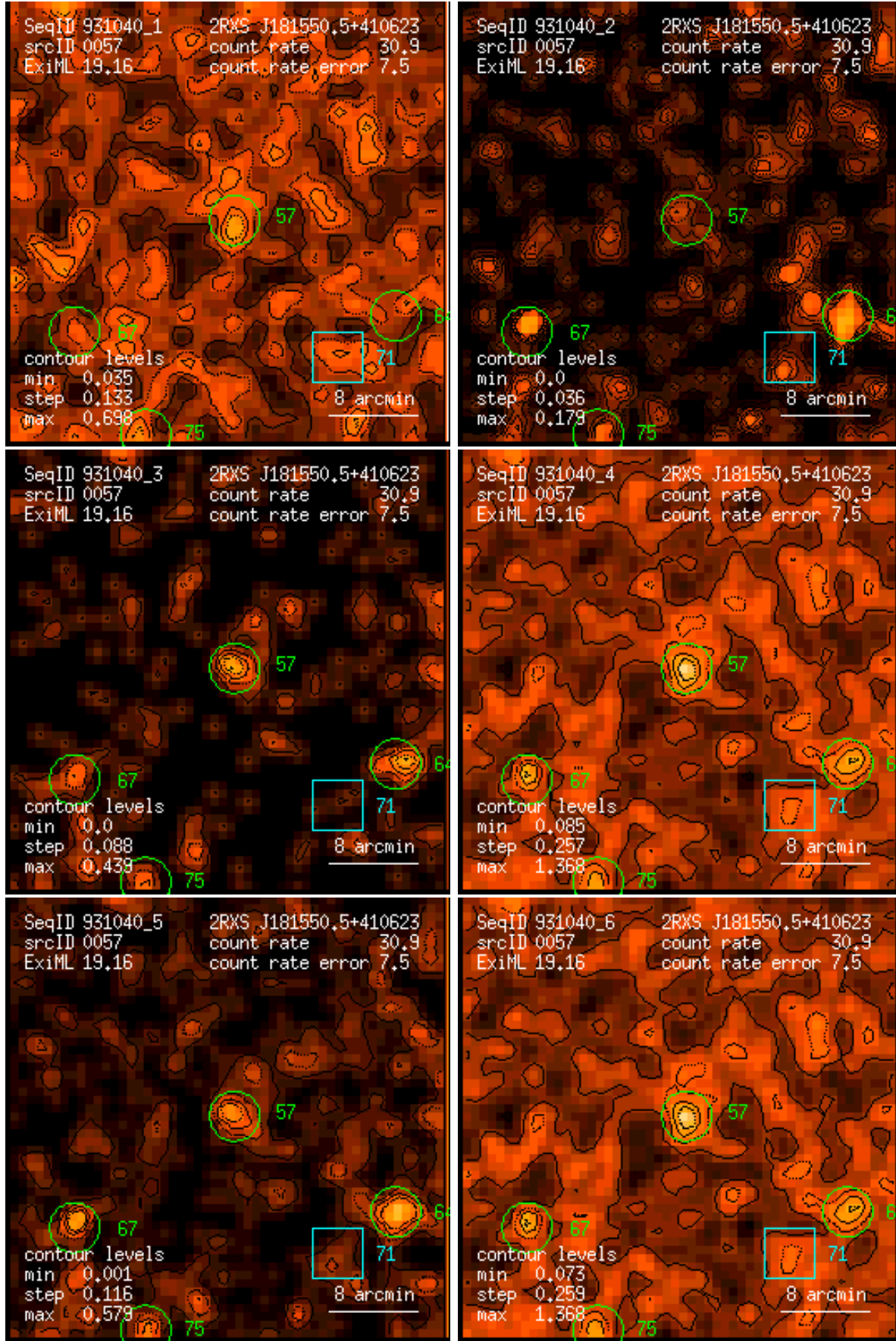
Figure 57: RASS 931040: detection 0057: band rate images, Gaussian filter: (1) PSPC channels 11 – 41, (2) 52 – 90, (3) 91 – 201, (4) 11 – 235, (5) 52 – 201, (6) 11 – 201. Broad band rates in counts/ks. Band rate contour levels in counts/ks/arcmin 2 .
