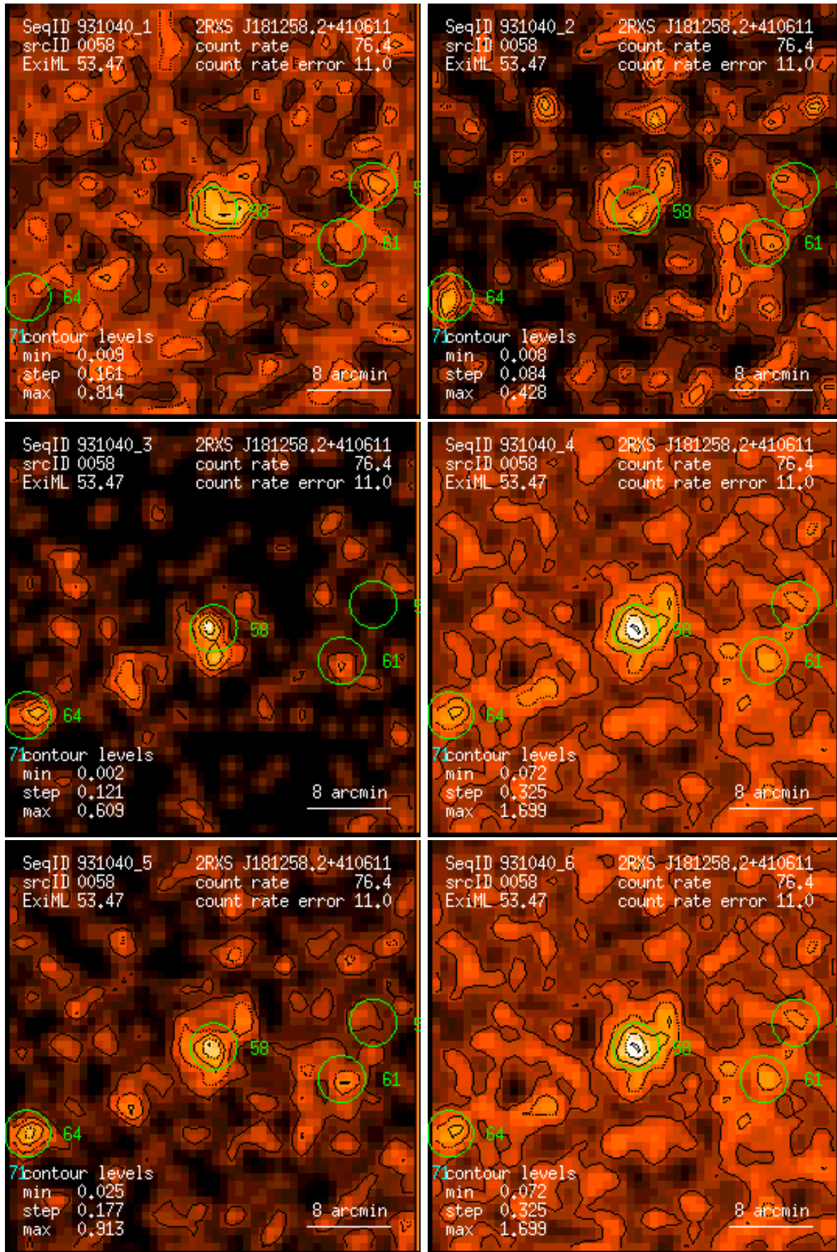
Figure 58: RASS 931040: detection 0058: band rate images, Gaussian filter: (1) PSPC channels 11 – 41, (2) 52 – 90, (3) 91 – 201, (4) 11 – 235, (5) 52 – 201, (6) 11 – 201. Broad band rates in counts/ks. Band rate contour levels in counts/ks/arcmin 2 .
