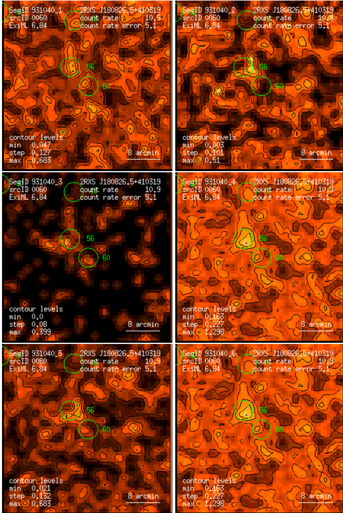
Figure 60: RASS 931040: detection 0060: band rate images, Gaussian filter: (1) PSPC channels 11 – 41, (2) 52 – 90, (3) 91 – 201, (4) 11 – 235, (5) 52 – 201, (6) 11 – 201. Broad band rates in counts/ks. Band rate contour levels in counts/ks/arcmin 2 .
