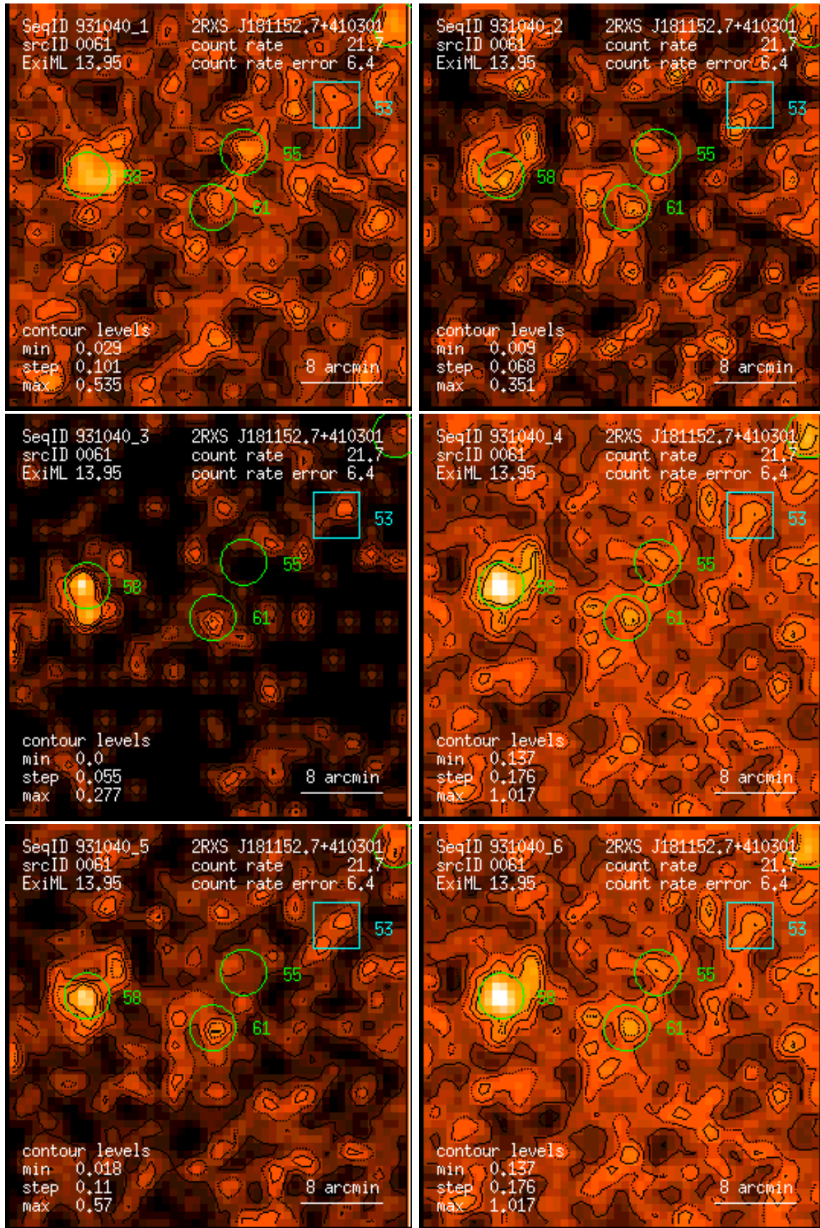
Figure 61: RASS 931040: detection 0061: band rate images, Gaussian filter: (1) PSPC channels 11 – 41, (2) 52 – 90, (3) 91 – 201, (4) 11 – 235, (5) 52 – 201, (6) 11 – 201. Broad band rates in counts/ks. Band rate contour levels in counts/ks/arcmin 2 .
