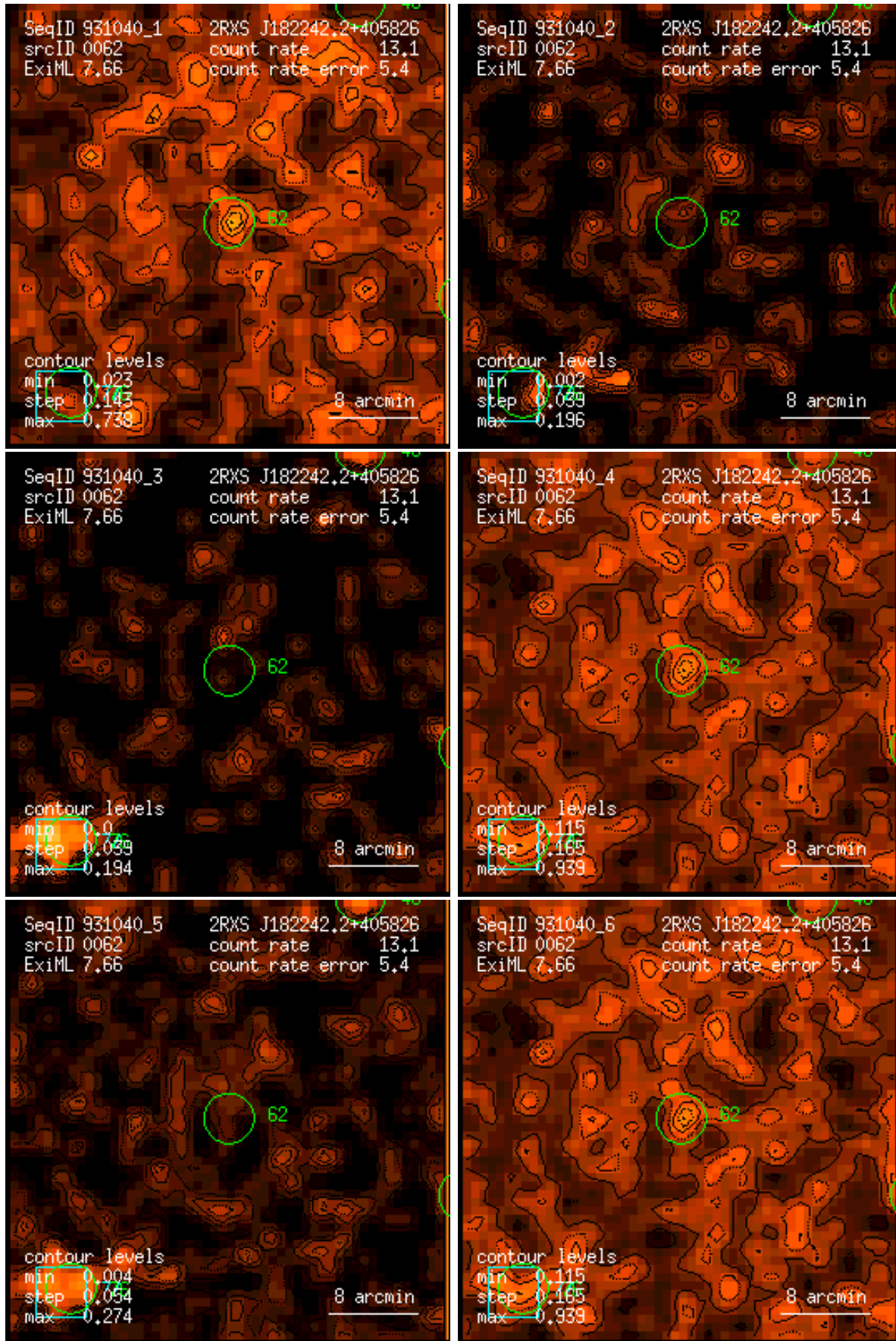
Figure 62: RASS 931040: detection 0062: band rate images, Gaussian filter: (1) PSPC channels 11 – 41, (2) 52 – 90, (3) 91 – 201, (4) 11 – 235, (5) 52 – 201, (6) 11 – 201. Broad band rates in counts/ks. Band rate contour levels in counts/ks/arcmin 2 .
