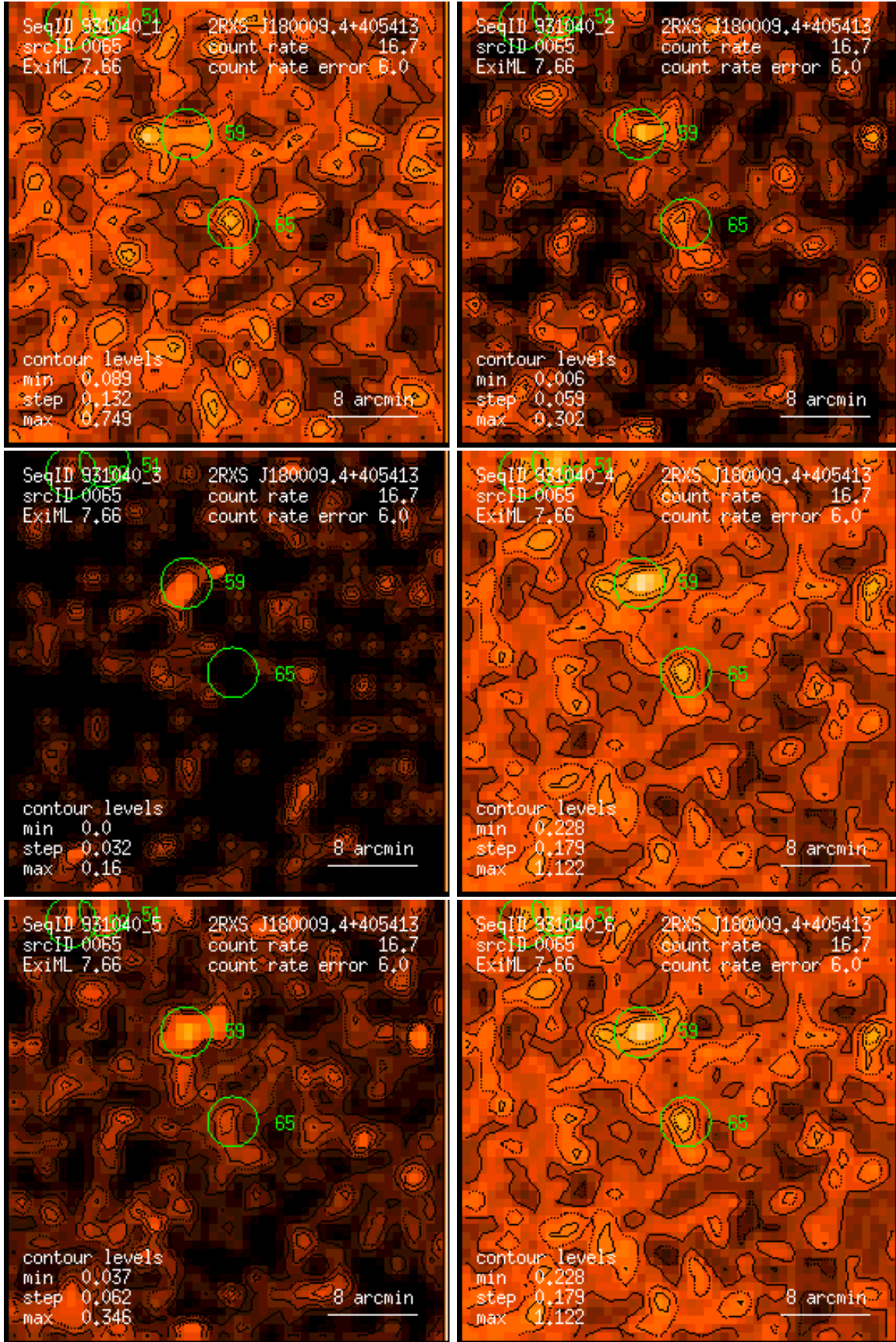
Figure 65: RASS 931040: detection 0065: band rate images, Gaussian filter: (1) PSPC channels 11 – 41, (2) 52 – 90, (3) 91 – 201, (4) 11 – 235, (5) 52 – 201, (6) 11 – 201. Broad band rates in counts/ks. Band rate contour levels in counts/ks/arcmin 2 .
