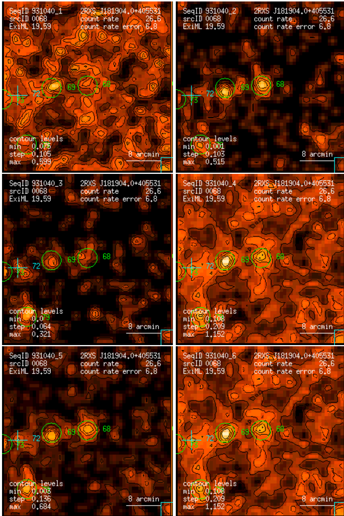
Figure 68: RASS 931040: detection 0068: band rate images, Gaussian filter: (1) PSPC channels 11 – 41, (2) 52 – 90, (3) 91 – 201, (4) 11 – 235, (5) 52 – 201, (6) 11 – 201. Broad band rates in counts/ks. Band rate contour levels in counts/ks/arcmin 2 .
