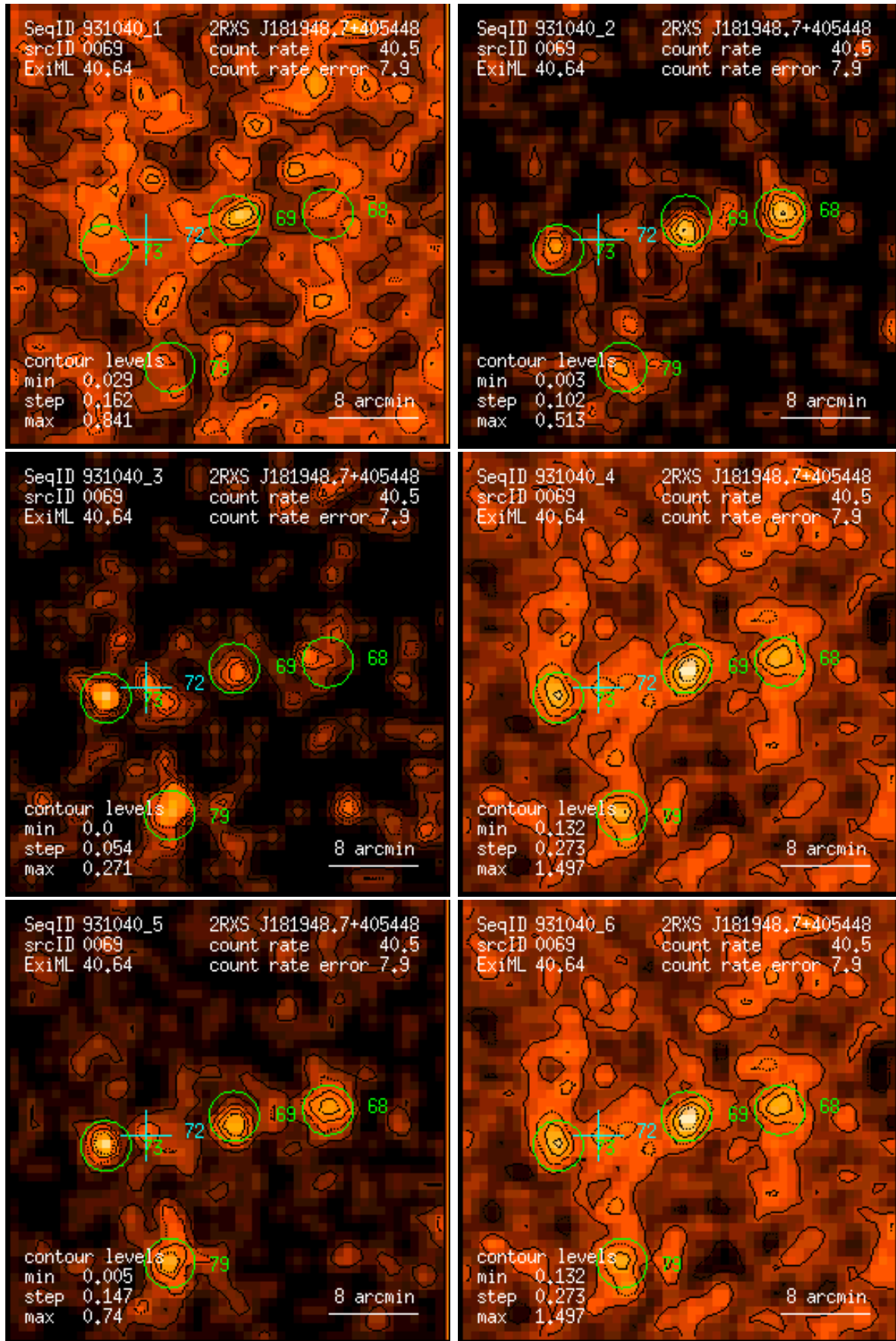
Figure 69: RASS 931040: detection 0069: band rate images, Gaussian filter: (1) PSPC channels 11 – 41, (2) 52 – 90, (3) 91 – 201, (4) 11 – 235, (5) 52 – 201, (6) 11 – 201. Broad band rates in counts/ks. Band rate contour levels in counts/ks/arcmin 2 .
