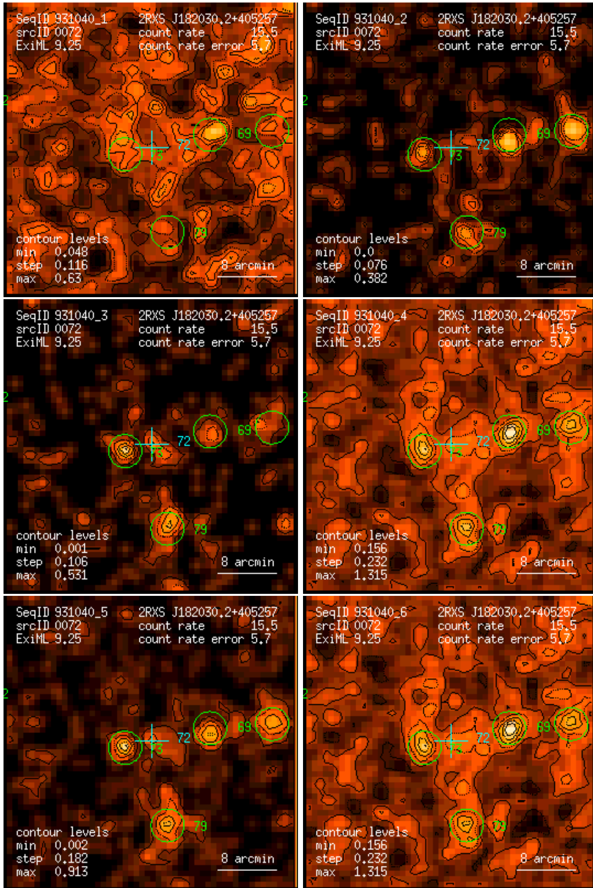
Figure 72: RASS 931040: detection 0072: band rate images, Gaussian filter: (1) PSPC channels 11 – 41, (2) 52 – 90, (3) 91 – 201, (4) 11 – 235, (5) 52 – 201, (6) 11 – 201. Broad band rates in counts/ks. Band rate contour levels in counts/ks/arcmin 2 .
