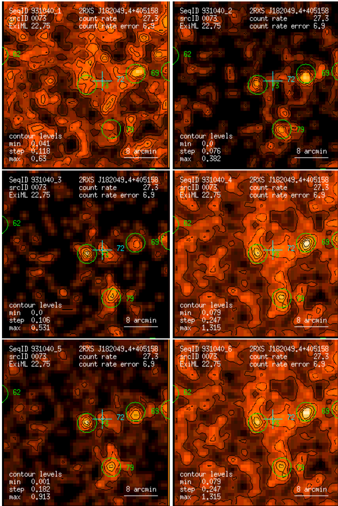
Figure 73: RASS 931040: detection 0073: band rate images, Gaussian filter: (1) PSPC channels 11 – 41, (2) 52 – 90, (3) 91 – 201, (4) 11 – 235, (5) 52 – 201, (6) 11 – 201. Broad band rates in counts/ks. Band rate contour levels in counts/ks/arcmin 2 .
