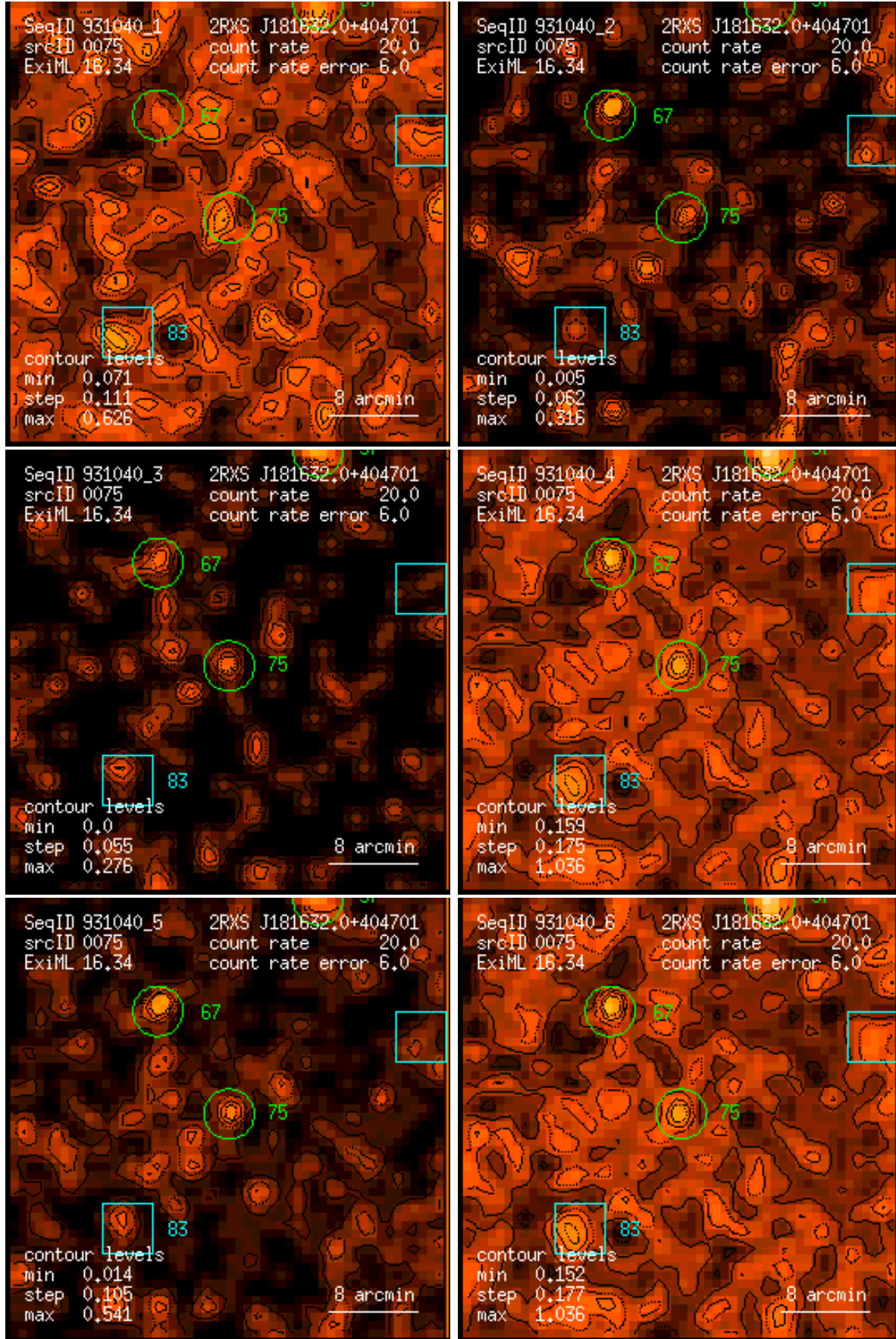
Figure 75: RASS 931040: detection 0075: band rate images, Gaussian filter: (1) PSPC channels 11 – 41, (2) 52 – 90, (3) 91 – 201, (4) 11 – 235, (5) 52 – 201, (6) 11 – 201. Broad band rates in counts/ks. Band rate contour levels in counts/ks/arcmin 2 .
