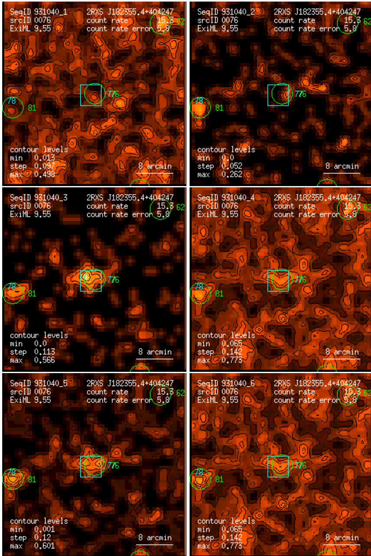
Figure 76: RASS 931040: detection 0076: band rate images, Gaussian filter: (1) PSPC channels 11 – 41, (2) 52 – 90, (3) 91 – 201, (4) 11 – 235, (5) 52 – 201, (6) 11 – 201. Broad band rates in counts/ks. Band rate contour levels in counts/ks/arcmin 2 .
